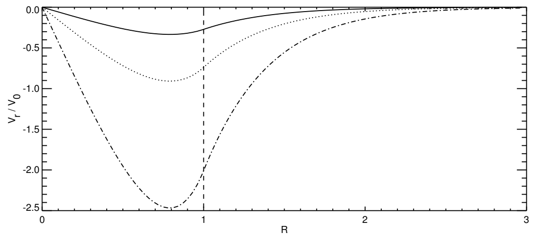
Figure 2. V_r/V_0(R) . Solid, dot and dash–dot lines correspond to \gamma t = 1, 2, 3 , respectively. r_0/L = 0.1 .
