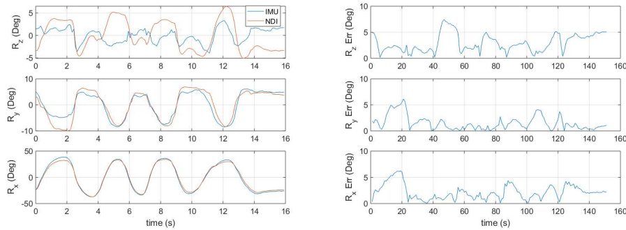
(a) Finger joint angles extracted from IMU sensors and NDI Polaris system. (b) Joint angle error with respect to NDI Polaris system.
