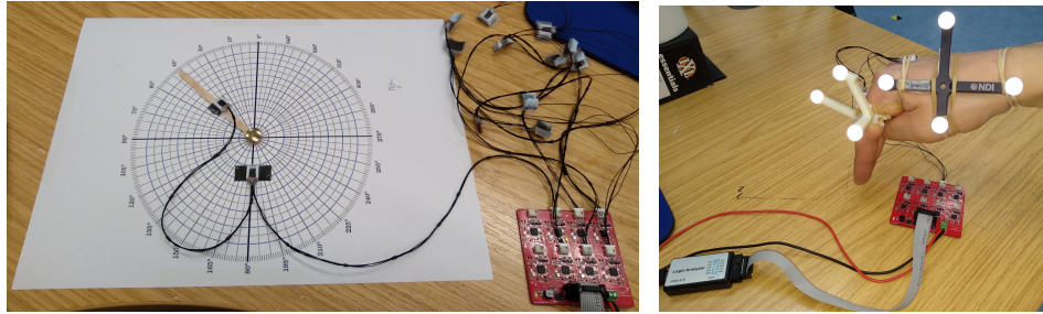
(a) Accuracy assessment setup in planar mode. (b) Accuracy assessment in 3D space.
