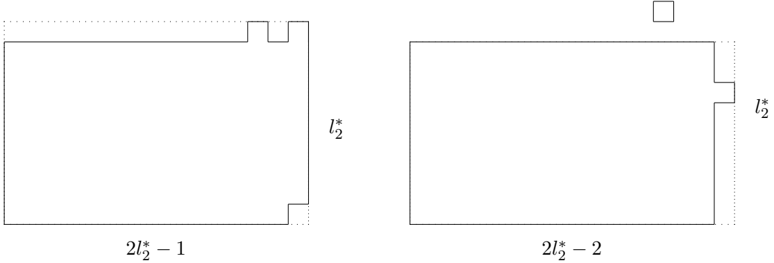
Figure 2: Configurations in \mathcal{P} : on the left hand-side is represented a configuration in \mathcal{P}_1 and on the right hand-side a configuration in \mathcal{P}_2
