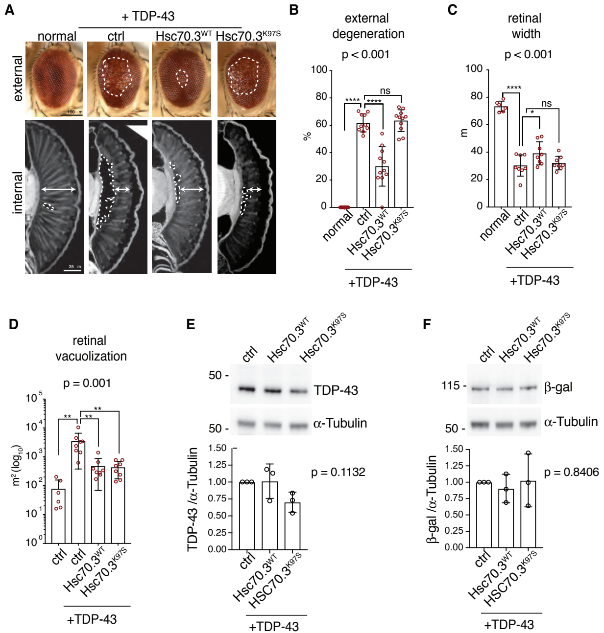
Figure 5: Hsc70.3 genetically interacts with TDP-43 in the Drosophila eye. A. Compared to the normal control, expression of human TDP-43 (ctrl) in the Drosophila eye leads to disruption of the external eye (white hatched line, top panel) and degeneration of the internal retina (white double headed arrow, and white hatched line lower panel). B. Expression of Hsc70.3 suppresses TDP-43-induced disruption of the external eye. Mean ( \pm SD), one way ANOVA and a Fisher's LSD test. ****: P<0.0001 and ns: not significant. C. Expression of Hsc70.3 WT suppresses TDP-43-induced reduction of retinal width (see double
