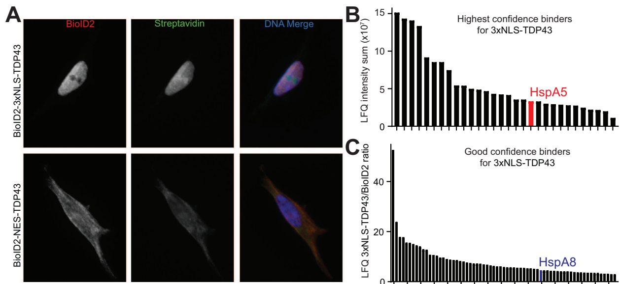
Figure 1: BioID of TDP-43 in SH-SY5Y cells in the nucleus and cytoplasm. A. Epifluorescence images for validating fusion-protein (red) expression and promiscuous biotinylation (green) localization following the addition of biotin. The 144 nuclear interactions of the 3xNLS-TDP-43 sample were separated into “Highest confidence associations”, proteins found only in the BioID2-3xNLS-TDP43, and not at all in the
