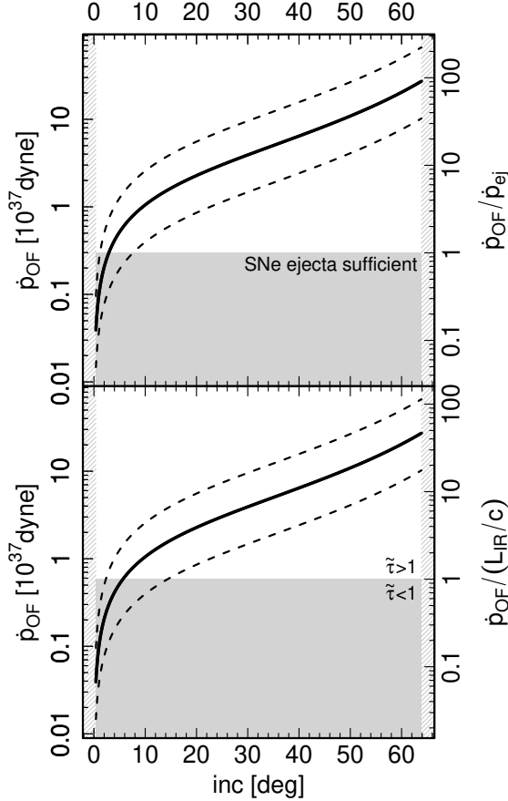
Figure 15. Deprojected momentum flux of the outflow \dot{p}_{OF} (left axes) as a function of inclination: Top: Comparing \dot{p}_{OF} to the momentum flux injected by SNe ejecta \dot{p}_{ej} (right axis) where the grey region indicates the momentum flux available from the estimated SNe rate \sim 15 SNe \text{yr}^{-1} . Bottom: Comparing \dot{p}_{OF} to the possible momentum flux contributed by radiation pressure from young stars on outflow dust grains. Values on the right axis indicate the required effective IR optical depth for a given \dot{p}_{OF} where the optically thin regime is indicated by the grey region. The 1\sigma spread in the \text{OH}^+ abundance modelled by Bialy et al. (2019) is shown by the dark gray shading and the upper and lower dashed lines indicate the \dot{E}_{OF} if the highest and lowest observed \text{OH}^+ abundances from Milky Way sightlines are assumed, respectively (Bialy et al. 2019). An outflow flowing perpendicular to the line of sight has an inc = 90^\circ . Hatched regions indicate regions outside of the considered inclination range.
