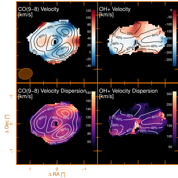
Figure 3. Top Left: Image plane velocity map of the CO(9-8) emission produced via a single Gaussian fitting procedure described in the text. Top Right: Image plane velocity map of the \text{OH}^+(1_1 - 1_0) blue-shifted absorption component, produced via a double, Gaussian fitting procedure described in the text. Bottom Left: Image plane velocity dispersion map of the CO(9-8) emission produced via a single Gaussian fitting procedure described in the text. Bottom Right: Image plane velocity dispersion map of the \text{OH}^+(1_1 - 1_0) blue-shifted absorption component produced via a double Gaussian fitting procedure described in the text. The beam ( 0.52'' \times 0.41'' ) is shown by the faded orange ellipse in the bottom left corner of the upper left panel. Contours indicate flux levels at 20%, 40%, 60% and 80% of the peak flux and optical depth of the CO(9-8) and \text{OH}^+ spectral lines, respectively.
