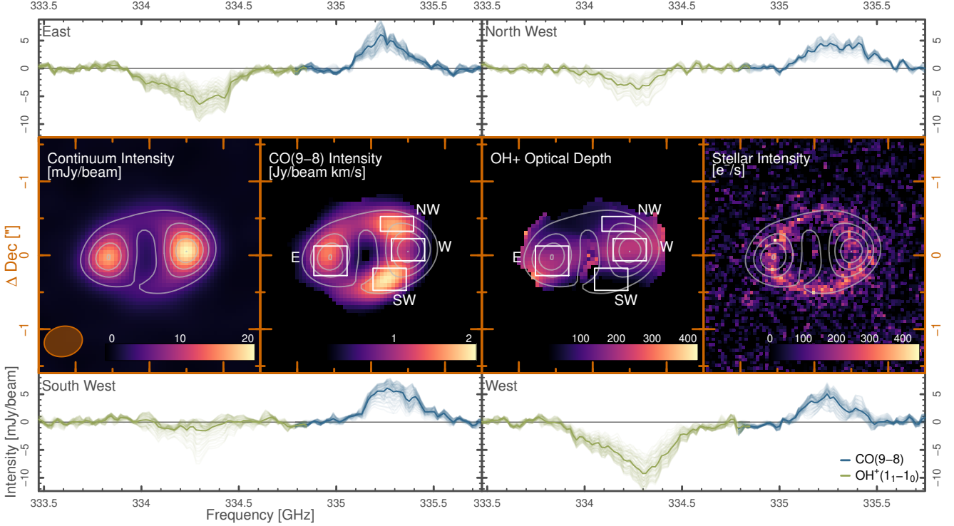
Figure 1. Middle Row - Far Left Panel: rest-frame 1034 GHz dust continuum emission observed with ALMA. The peak of the dust emission is lensed into a prominent double image configuration with a brighter western image, accompanied by a complete Einstein ring. The synthesized beam ( 0.52'' \times 0.41'' ) is shown by the faded orange ellipse in the bottom left. The grey contours indicate continuum levels of 20%, 40%, 60%, 80% and 100% that of the peak and are overlaid in the following three panels. Middle Row - Center Left Panel: Intensity map of the rest-frame 1036.9 GHz CO(9-8) emission line observed with ALMA, produced via a single Gaussian fitting procedure. The CO(9-8) emission reveals itself in 3 distinctly different peaks compared to the continuum but again accompanied by a complete Einstein ring. Middle Row - Center Right Panel: Integrated optical depth map of the blue-shifted component of the \text{OH}^+(1_1 - 1_0) absorption line observed with ALMA, produced via a double Gaussian fitting procedure. The peak \text{OH}^+ optical depth is approximately cospatial with the peaks in the continuum emission albeit with an elongated morphology stretching from East to West. Middle Row - Far Right Panel: Keck Ks ( \lambda = 2.2 \mu\text{m} ) stellar intensity map with the lens subtracted (Calanog et al. 2014). As in the continuum and CO(9-8) emission, a distinct Einstein ring is observed, but with gaps at the positions of peak FIR continuum emission. Outer 4 Panels: Each of the four outer panels correspond to a region with a matching label (E: East, NW: North West, SW: South West, W: West) indicated by the solid white boxes in the central two panels and are placed over peaks in the continuum and CO(9-8) emission. The outer panels display continuum subtracted CO(9-8) and \text{OH}^+ spectra of the individual spaxels (pixel area = 0.05'' \times 0.05'' ) of each region in transparent blue and green, respectively. The average spectra of each region are shown by the solid line. The CO(9-8) and \text{OH}^+ spectra do not display significant variation in spectral shape or central velocity between the four regions.
