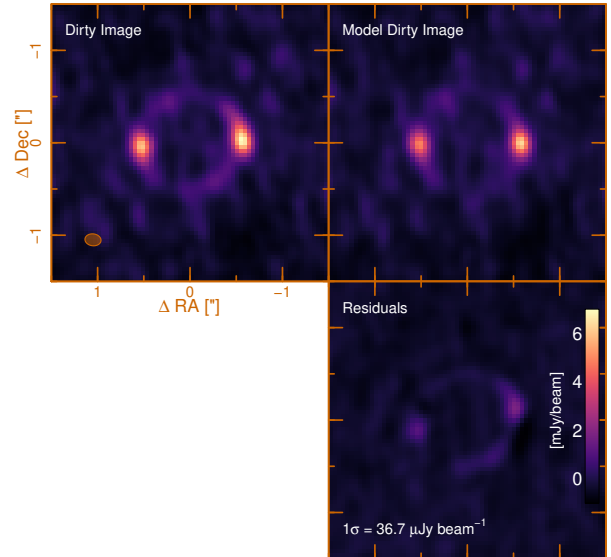
Figure 4. visilens modelling of the high spatial resolution CH + (1-0) continuum emission in G09v1.40. Top Left: Dirty image of the data with beam (0.17 '' x0.13 '' ) shown as the orange ellipse in the bottom left corner. Top Right: Dirty image of the visilens model, recovering 85% of the flux in the dirty image. Bottom: Residuals, with the rms beam -1 shown in the bottom left corner.
