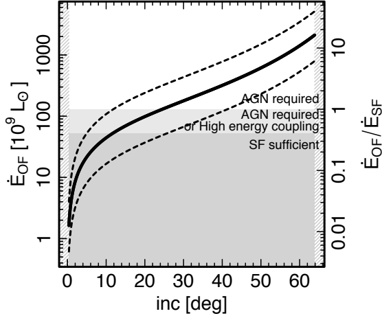
Figure 14. Deprojected outflow kinetic energy flux (kinetic luminosity) of the outflow \dot{E}_{\text{OF}} as a function of inclination (left axis) and normalised by the kinetic energy flux injected by SNe \dot{E}_{\text{SF}} (a.k.a. energy loading, right axis). The bottom grey region indicates the energy transferred to the ISM assuming an energy coupling up to 40%, which can occur if SNe are clustered. Higher \dot{E}_{\text{OF}} require either unusually high energy coupling or an AGN contribution. The upper and lower dashed lines indicate the \dot{E}_{\text{OF}} if the highest and lowest observed \text{OH}^+ abundances from Milky Way sightlines are assumed, respectively (Bialy et al. 2019). An outflow flowing perpendicular to the line of sight has an inc = 90^\circ . Hatched regions indicate regions outside of the considered inclination range.
