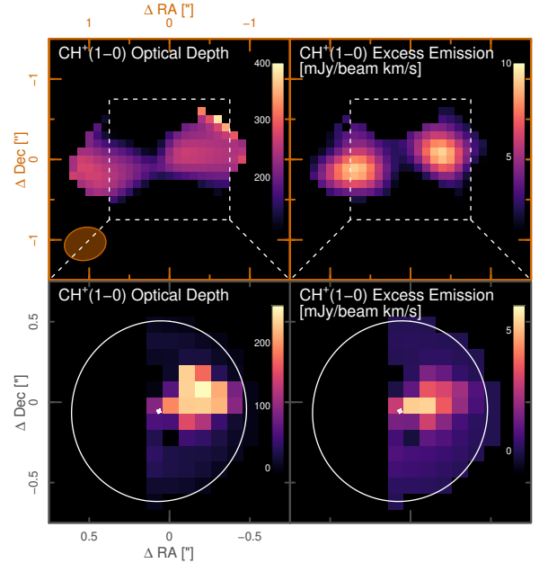
Figure 11. Top Row: Image plane maps of the \text{CH}^+(1-0) absorption line optical depth and excess \text{CH}^+(1-0) emission in the low-resolution \text{CH}^+ data set. The beam ( 0.59'' \times 0.46'' ) is displayed in the bottom left corner of the left-hand panel. Bottom Row: Source plane reconstructions of the above panels. Whilst the \text{CH}^+ optical depth map follows the \text{OH}^+ optical depth map morphology, the \text{CH}^+ emission follows more closely the dust continuum intensity distribution. Pixel area ( 0.1'' \times 0.1'' ) is the same in both the image and source planes.
