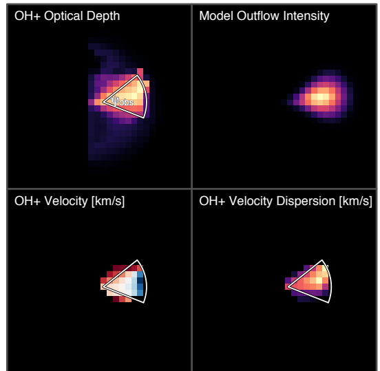
Figure 8. Example Conical outflow model compared to the observed OH + optical depth map. Top Left: Source plane OH + optical depth map with measured 2D projected cone geometry overlaid in white. The projected radius is denoted by R_{obs} and 2D projected opening angle by \Delta\phi . Top Right: 2D projection of a model conical outflow with constant radial density. Bottom Left: Source plane OH + line of sight velocity map with measured 2D projected cone geometry overlaid in white. Outflow velocity increases with radius. Bottom Right: Source plane OH + velocity dispersion map with measured 2D projected cone geometry overlaid in white. Outflow velocity dispersion increases with radius.
