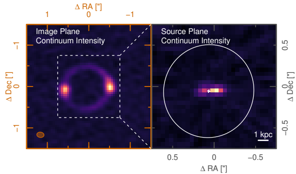
Figure 5. Source plane reconstruction of dust continuum emission from the ‘high’ spatial resolution \text{CH}^+(1-0) data set using LLENSTOOL. The left panel displays the observed image plane dust continuum intensity with the beam ( 0.17'' \times 0.13'' ) shown in the lower left by the shaded orange ellipse. The right panel is a zoom in of the white dashed region in the left panel, displaying the source plane reconstruction of the dust continuum. The lens caustics are indicated by the solid white lines and a physical scale of 1kpc is given in the lower right corner. A single compact and elongated source is revealed directly to the West of the inner caustic. The weak eastern feature is an artifact of beam smearing over the outer caustic in the image plane.
