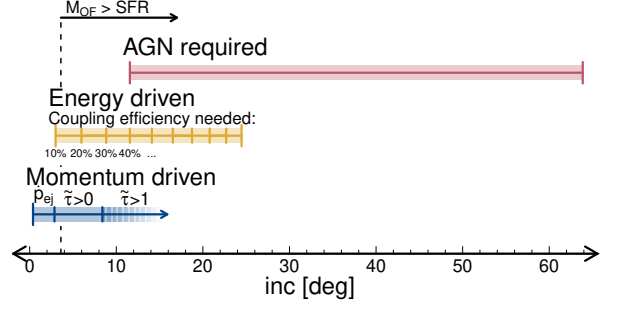
Figure 16. Possible outflow driving mechanisms as a function of outflow inclination. If the inclination is < 2.9^\circ the momentum provided by SNe ejecta is sufficient to drive the outflow through a momentum-driven phase (blue bar). If inc > 2.9^\circ a momentum-driven phase is still possible, if radiation pressure from young stars on dust grains in the outflow is non-negligible. This requires \tau_{\text{eff,IR}} > 0 and \tau_{\text{eff,IR}} > 1 if inc > 8.4^\circ . In the absence of radiation pressure, the outflow requires a momentum boost if inclinations are > 2.9^\circ , which can be provided by an energy-driven phase of the shocked SNe ejecta if thermal energy is not immediately and completely radiated away. The energy coupling required to drive the outflow via SNe feedback is indicated below the yellow bar. If the inclination is > 12^\circ the outflow requires either an unusually high energy coupling of > 40\% , which is higher than that expected from a clustered SNe scenario, or a contribution from a low-luminosity, obscured or fossil AGN (red bar). In reality, all driving mechanisms may be contributing simultaneously and if the full multiphase and double-sided outflow were to be taken into account the inclination ranges shown here would be shifted to smaller inclinations.
