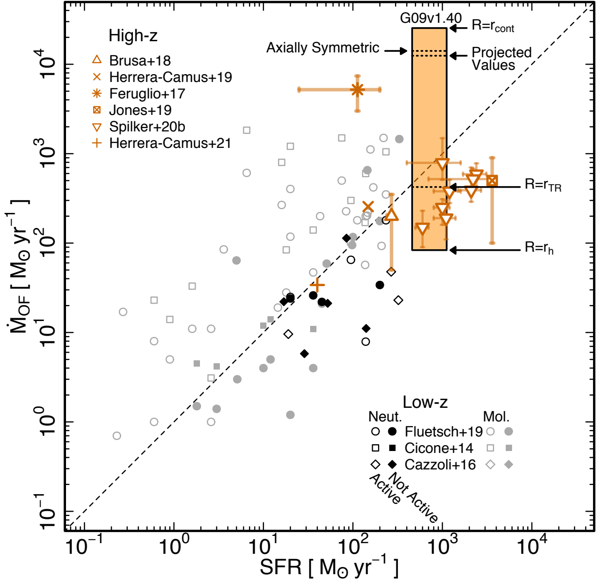
Figure 13. Mass outflow rate as a function of star formation rate. The shaded light orange region indicates the parameter space of the neutral gas outflow in G09v1.40 over the possible inclination range discussed in Sec. 7. We additionally indicate \dot{M}_{\text{OF}} s estimated for an axially symmetric galaxy with a perpendicular outflow (upper dashed line), using only projected outflow parameters (middle dashed line), and for an outflow with a radius equal to that of the turbulent reservoir surrounding G09v1.40 (Falgarone et al. 2017) (lower dashed line). For comparison we plot molecular and neutral gas outflows measured in local galaxy samples with grey and black symbols, respectively (Fluetsch et al. 2019; Cicone et al. 2014; Cazzoli et al. 2016). Open and filled symbols indicate sources with and without AGN activity, respectively. With orange symbols we show high redshift molecular outflows measured in the following sources, listing their galaxy type, outflow tracer and redshift in brackets: XID2028 (QSO, CO, z = 1.593 ; Brusa et al. 2018), zC400528 (AGN, CO, z = 2.387 ; Herrera-Camus et al. 2019), APM08279+5255 (QSO, CO, z = 3.912 ; Feruglio et al. 2017), SPT 0346-52 (DSFG, \text{H}_2\text{O} , z=5.656 ; Jones et al. 2019), and various SPT sources (DSFG, OH, z > 4 ; Spilker et al. 2020b). Also in orange, we include the neutral gas outflow in HZ4 (main-sequence star-forming galaxy, [CII], z \sim 5 Herrera-Camus et al. 2021).
