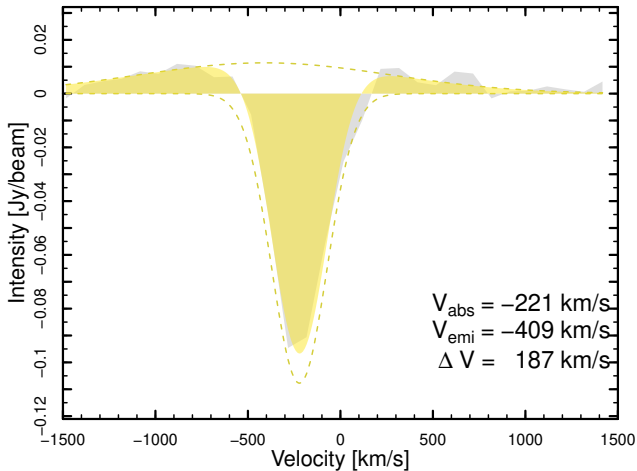
Figure 10. Stacked \text{CH}^+(1-0) spectra of all spaxels with continuum signal to noise > 3 , in the high spatial resolution data set. The spectra is fitted with two Gaussian components, shown separately with the dashed yellow lines and combined with the shaded yellow region. The blue-shifted absorption and emission lines reveal outflowing neutral and shocked gas with line of sight velocities of V_{\text{abs}} = -221 \text{ km s}^{-1} and V_{\text{emi}} = -409 \text{ km s}^{-1} , respectively. The strength of the \text{CH}^+ emission is much weaker, and its central velocity much more blue-shifted than previously reported by Falgarone et al. (2017) using the low spatial resolution data set.
