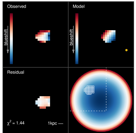
Figure 7. Example spherical outflow model compared to the observed \text{OH}^+(1_1 - 1_0) velocity map. The model suggests the outflow is ejected from outside the galaxy and is therefore ruled out. Top Left: Reconstructed and normalised velocity map of the observed outflow in \text{OH}^+ . Top Right: Spatially averaged model velocity map from region in the dashed box in the panel below. The yellow marker indicates the ejection location predicted by this model. Bottom Left: Residual velocity map of the normalised model velocity map and normalised \text{OH}^+ velocity map. Bottom Right: Full 2D LOS velocity map of the spherical outflow model with a dashed box outlining the edges of the panel above.
