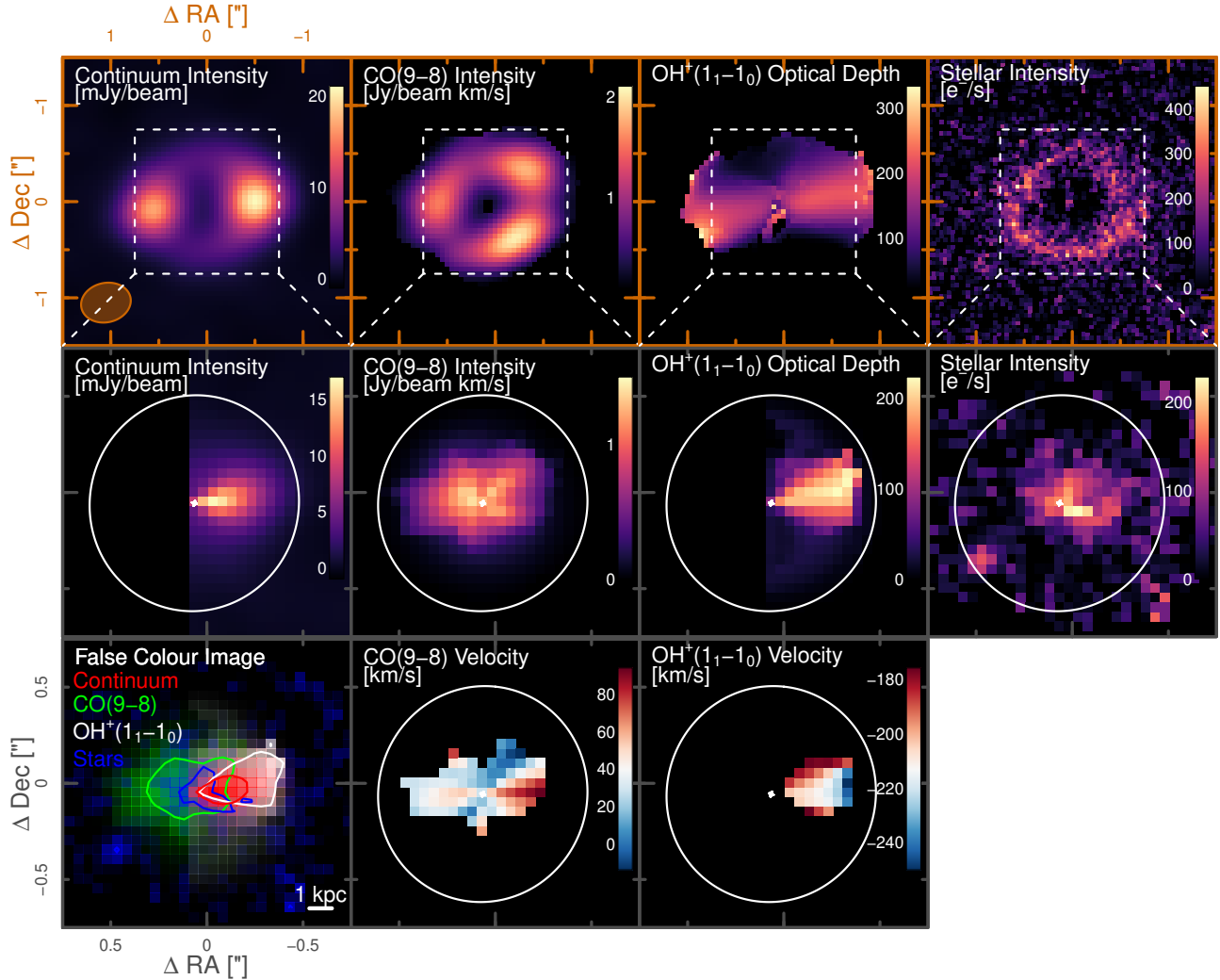
Figure 6. ALMA Cycle 3 observations of the gravitationally lensed galaxy H-ATLAS J085358.9+015537 at redshift z = 2.09 . Row 1: Image plane intensity maps of the dust continuum, CO(9-8) emission tracing the warm dense gas in the disk, \text{OH}^+(1_1 - 1_0) optical depth tracing neutral outflowing gas and Keck Ks band stellar emission. The beam ( 0.52'' \times 0.41'' ) is shown in the bottom left corner of the left-hand panel. Row 2: Reconstructed source plane intensity maps of the components shown in row 1. Lensing caustics are shown in white. Row 3 Left panel: False colour image of all the source plane intensity maps of the dust (red), CO(9-8) (green), \text{OH}^+ (white) and stars (blue). A single contour of each distribution is drawn at 60% of their respective peak values. Row 3: Reconstructed source plane velocity maps. The second panel shows the velocity map of the CO(9-8) emission and the third panel shows the \text{OH}^+ velocity field. The first panel is the \text{OH}^+ velocity map minus the CO(9-8) velocity map which, if the outflow was a flat sheet of gas lifting off the galaxy disk, should be uniform. This is clearly not the case and this scenario is therefore ruled out (See Sec. 5.1). Pixel area ( 0.05'' \times 0.05'' ) is the same in both the image and source planes and a source plane physical scale of 1kpc is given in the lower right corner of the last panel.
