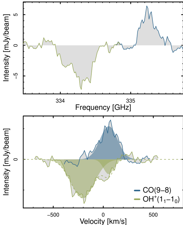
Figure 2. Continuum subtracted \text{OH}^+(1_1 - 1_0) absorption (green) and \text{CO}(9-8) emission (blue) spectra in a single ALMA spaxel (pixel area = 0.05'' \times 0.05'' ) observed simultaneously in the DSFG G09v1.40. Top: Spectra plotted as a function of observed frequency. Bottom: Spectra plotted as a function of velocity with respect to the galaxy’s systemic velocity determined from the z=2.0924 redshift measurement by Yang et al. (2017). We fit the \text{OH}^+(1_0 - 1_1) absorption and \text{CO}(9-8) emission lines with double and single Gaussian functions, respectively; the shaded regions of the same colour indicate the individual Gaussian components to each spectral line, whilst the dashed green line presents the full \text{OH}^+ fit. The main \text{OH}^+ component is blue-shifted \sim 200 \text{ km s}^{-1} with respect to the bulk molecular gas as traced by the \text{CO}(9-8) emission, revealing a neutral outflow at these velocities. Note also the larger width of the \text{OH}^+ line.
