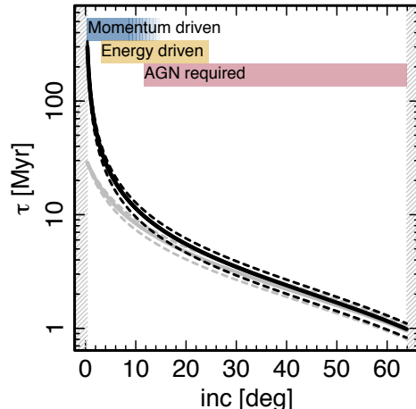
Figure 17. Depletion time of the host galaxy’s gas reservoir given the observed neutral gas mass outflow rate (black lines), and in combination with the SFR (grey lines), as a function of possible outflow inclination. The upper and lower dashed lines (black and grey) indicate the depletion time if the highest and lowest observed \text{OH}^+ abundances from Milky Way sightlines are assumed, respectively (Bialy et al. 2019). The outflow driving mechanisms from Fig. 16 are shown at the top. An outflow flowing perpendicular to the line of sight has an \text{inc} = 90^\circ . Hatched regions indicate regions outside of the considered inclination range.
