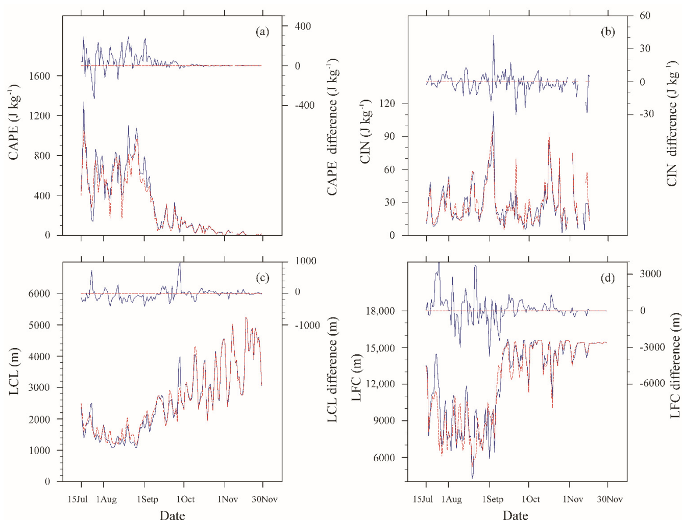
Figure 10. Temporal variations of the TRSR basin averaged values for the boundary layer elements (a) CAPE, (b) CIN, (c) LCL, (d) LFC. The curve on the lower half corresponds to the Y-axis on the left, with the red line representing WRF-H and the blue line representing WRF-S. The curve on the upper half corresponds to the y-axis on the right side, and the red line represents the bias of WRF-H relative to WRF-S.
