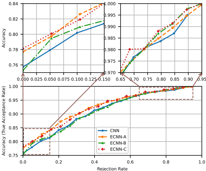
Fig. 4. The mean ARC plots of all models under CV scheme when considering the ‘overall’ uncertainty estimate.
