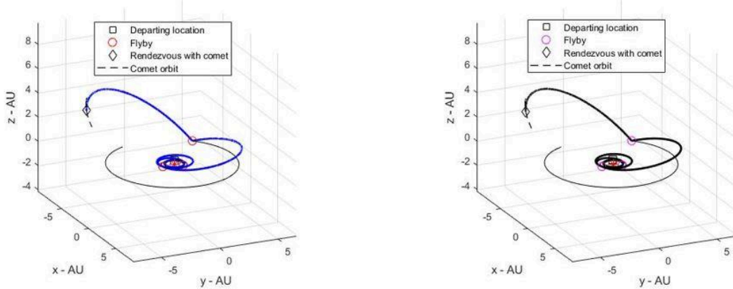
Fig. 21 3D representation of a long transfer to 2017/R1 employing an EVECJ sequence. Left plot is obtained with defects formulation, while right plot with DSMs formulation. From innermost to outermost, black circles represent Venus, Earth, and Jupiter orbits, respectively.
