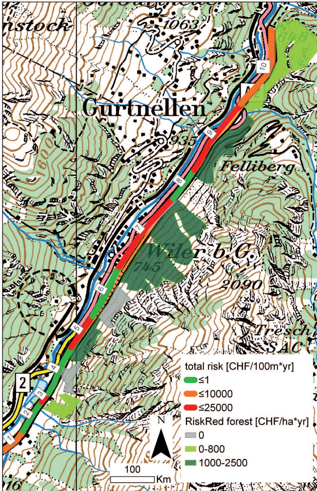
Figure 3. Total risk with the current forest along the considered highway section, and risk reduction provided by the protection forest complexes.
