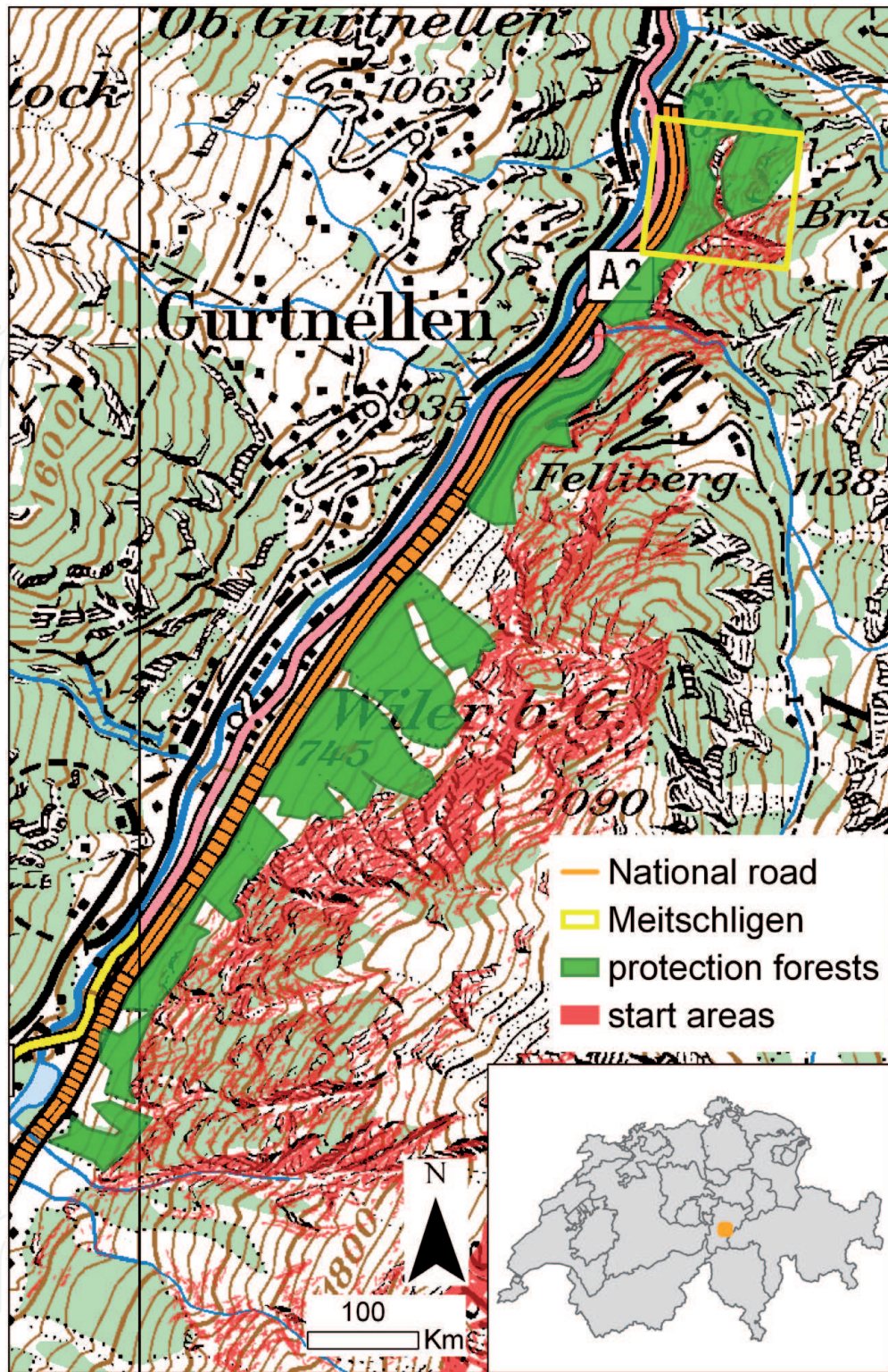
Figure 2. Study region along the A2 Gotthard highway with protection forest complexes and release area and the local case study site in Meitschlingen.
