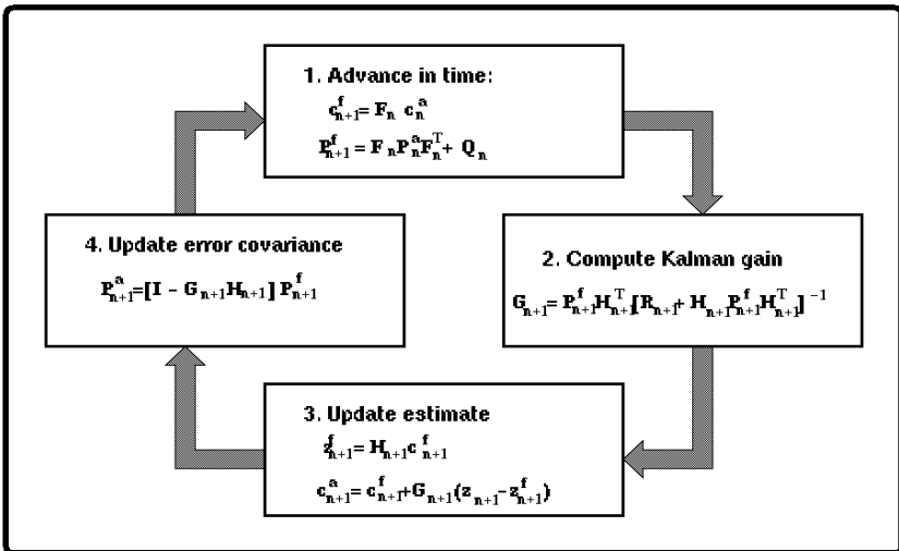
Fig. 1. A sketch for linear Kalman filter.
