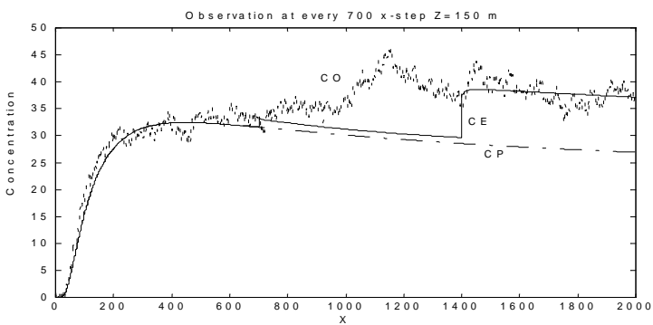
Fig. 2. Effect of the observation frequency in the KF: (a) EXP3; (b) EXP5; (c) EXP6.
