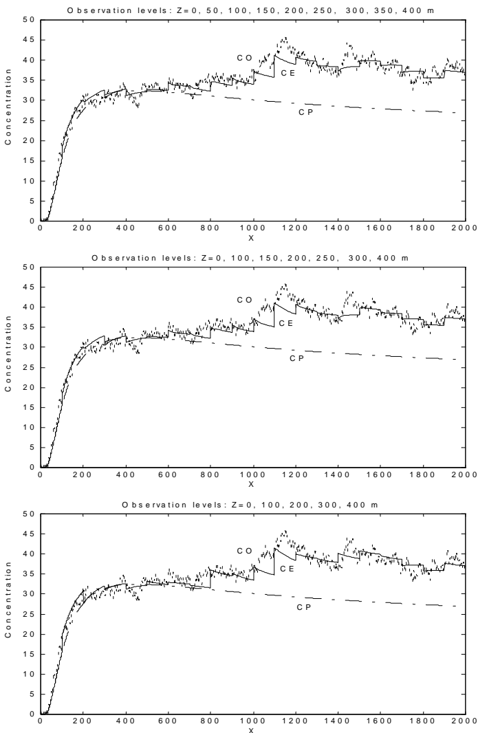
Fig. 3. Assimilation with different observation grids: (a) N_m = 9 , (b) N_m = 7 , (c) N_m = 5 .
