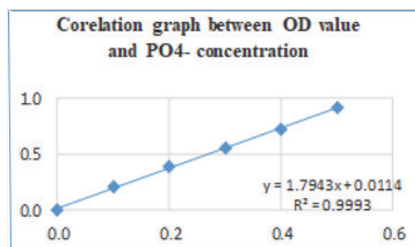
Figure 4. Correlation graph between OD value and PO 4 - concentration
