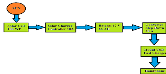
Gambar 2. Blok diagram proses perancangan station charger handphone
