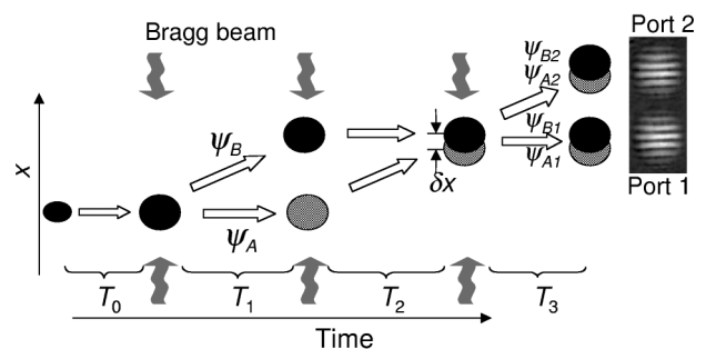
FIG. 1. Space-time diagram of the experiment. Three optically induced Bragg-diffraction pulses form the interferometer. The condensate is released for a time T_0 before the first Bragg pulse. The centers of \psi_A and \psi_B are separated by \delta x at the time of the third Bragg pulse, which splits them into \psi_{A1} , \psi_{B1} , and \psi_{A2} , \psi_{B2} . Before imaging the atoms, we allow the output ports to separate for a time T_3 \approx 2 ms. The image shows the output ports when T_0 = 3 ms, T_1 = 1 ms, and T_2 = 1.3 ms.
