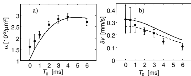
FIG. 4. (a) Plot of the phase curvature \alpha versus the initial expansion time T_0 showing the phase evolution from mean-field expansion. The solid line is a calculation using the Lagrangian variational method (LVM). (b) Plot of the relative repulsion velocity \delta v versus T_0 . The solid curve is the calculated maximum repulsion velocity (when \delta x = 0 ) and the dashed curve is the repulsion velocity averaged over the range of \delta x used in the experiment.
