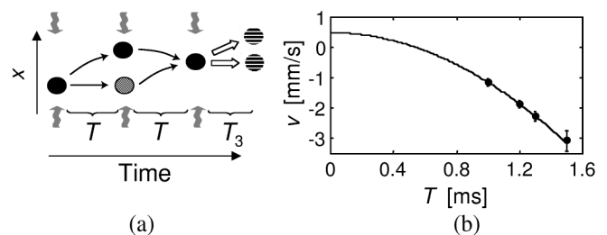
FIG. 5. (a) Schematic representation of the interferometer in the trap, with the principle difference from Fig. 1 being the curved arrows indicating the acceleration of the wave packets. (b) The relative velocity v between the two trapped wave packets versus the interferometer time T . The solid line is a fit.
