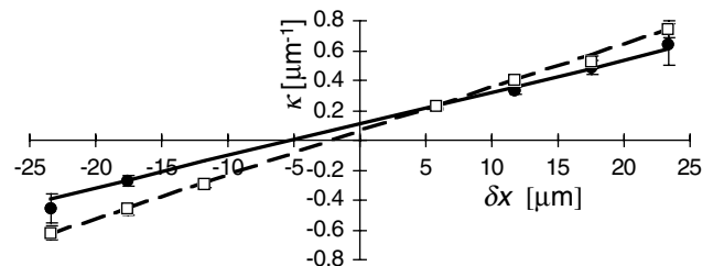
FIG. 3. Plot of the spatial fringe frequency \kappa versus \delta x for T_0 = 1 ms (filled circles) and 4 ms (open squares). The solid and dashed lines are linear fits to the data.
