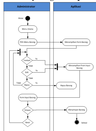
Gambar 3.4 Activity Diagram Input Barang
