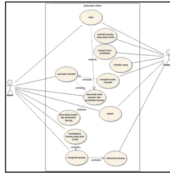
Gambar 3.1 Use Case Diagram
