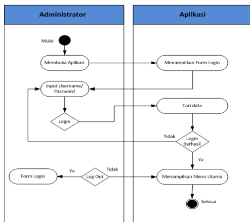
Gambar 3.3 Activity Diagram Login Admin
