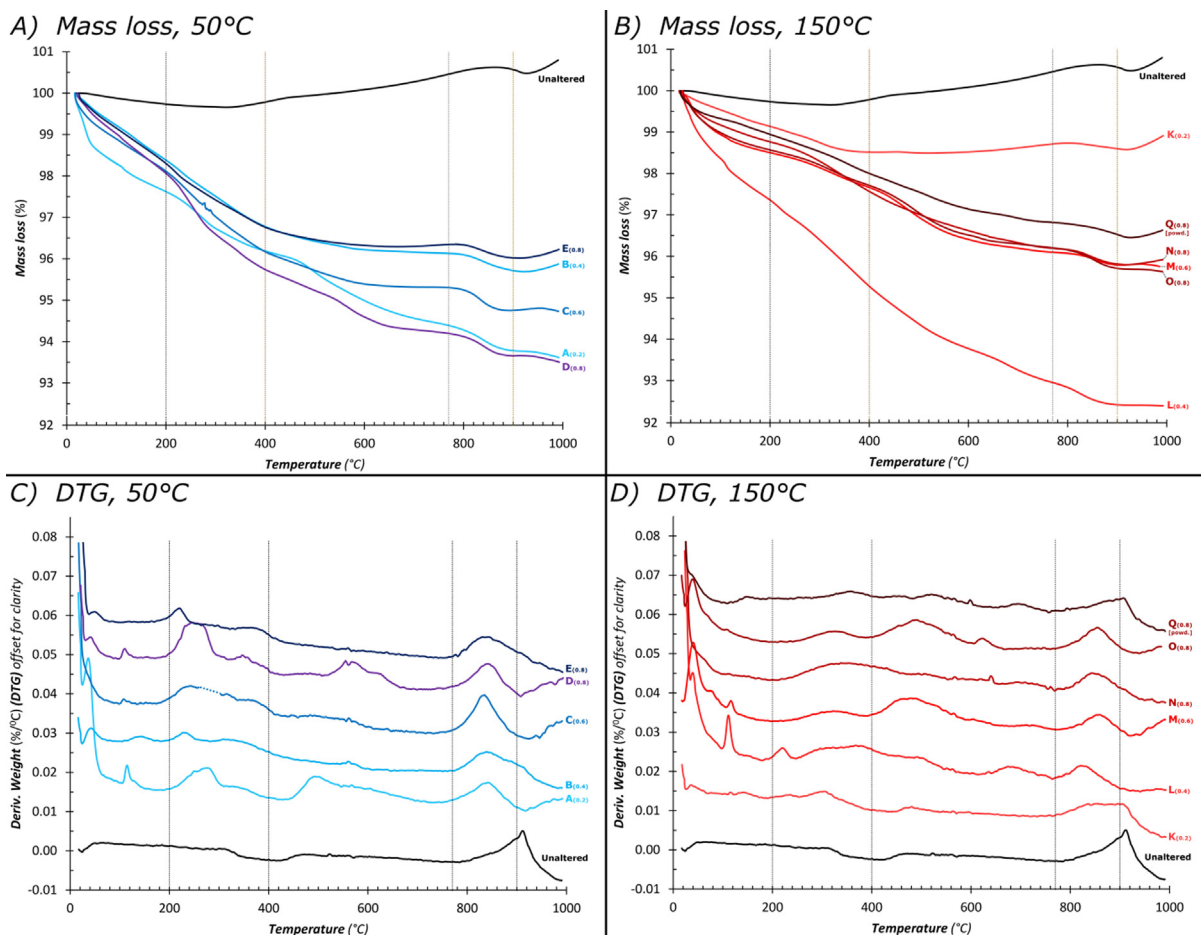
Fig. 7. Thermogravimetric data illustrating temperature-dependent mass loss due to the release of volatile gases from the altered samples upon heating from room temperature ( \sim 20 °C) to 1000 °C. Volatile gasses are emitted as mineral phases thermally decompose. Low-temperature (50 °C) analyses (panels A and C) are shown in blue, while high-temperature (150 °C) samples (panels B and D) are shown in red. Panels A and B display mass loss as a function of temperature, while panels C and D display the differential thermogravimetry curves for each sample. The response of the unaltered Kainsaz is shown in black for reference. Peaks in the DTG curves indicate the thermal decomposition of specific mineral phases. Vertical dashed lines, located at 200 °C, 400 °C, 770 °C and 900 °C correspond to the ranges and boundaries conventionally attributed to the decomposition of volatiles from adsorbed water, Fe-oxyhydroxides, phyllosilicates, and carbonates respectively (as detailed in Garenne et al., 2014 ).
