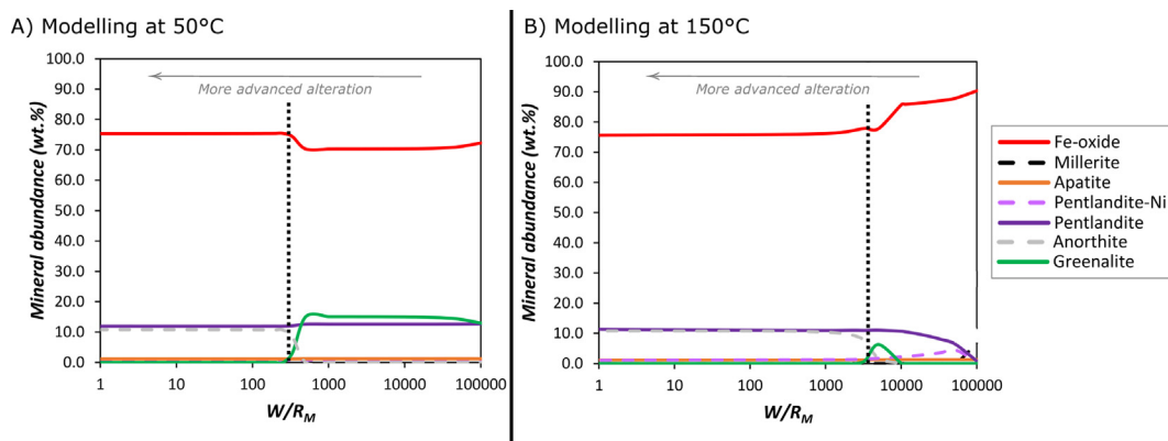
Fig. 10. Modelled secondary mineral assemblages formed in equilibrium at (A) 50 °C and (B) 150 °C. Vertical dashed lines indicate the inferred effective W/R , that is the amount of rock that is inferred to have reacted with fluids. These values are approximately 250 for the 50 °C experiments and 3300 for the 150 °C experiments.
