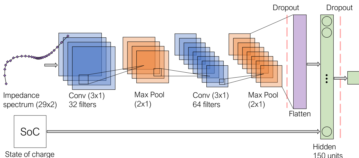
Figure 1. Diagram of the convolutional neural network architecture employed for direct estimation of state of health using impedance spectroscopy measurements—with the real and imaginary components of the battery impedance at each sampling frequency forming a 29 \times 2 input matrix, respectively—and battery state of charge.
