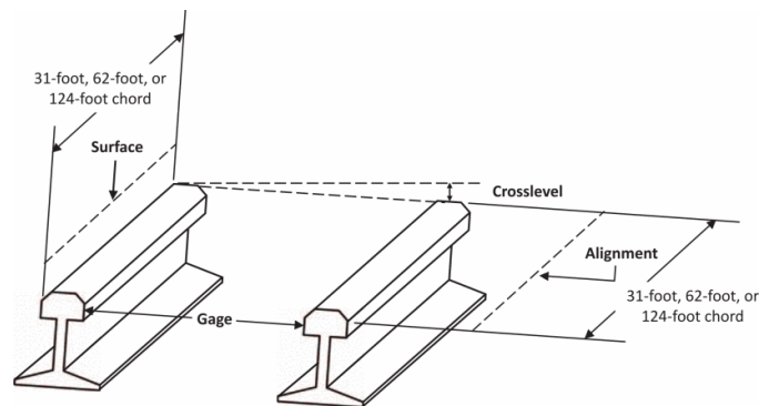
Figure 1 Track geometry 5
