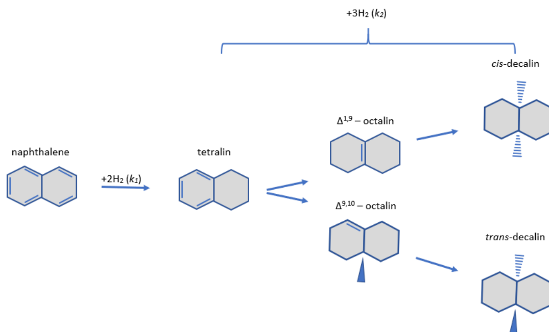
Scheme 1. Naphthalene hydrogenation reaction pathways.
