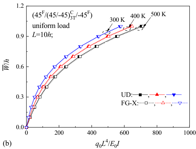
Figure 16: Effect of thermal field on bending behavior of hybrid laminated plates.
