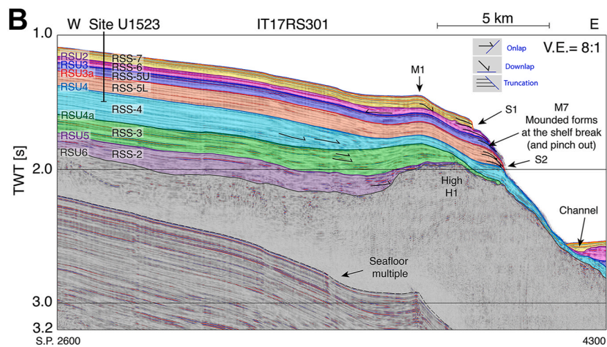
Fig. 7. Seismic section IT17RS301 in seconds Two-Way travel Time (TWT). a) uninterpreted section; b) interpreted section. Location of the International Ocean Discovery Program (IODP) Site U1523 is shown. The scarps are S1 and S2, M1 is the contouritic mound. M7 labels a contouritic deposit at the shelf break. Location of the section is shown in Fig. 2.
