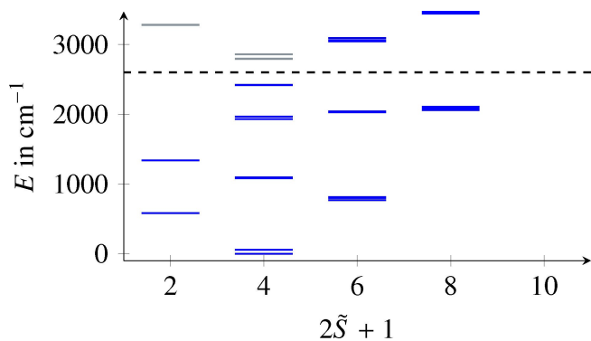
Figure 2. CASOCI energies (with shift) of the trinuclear Co II V II Co II system, mapped to pseudo-spin multiplicities. Above \sim 2600 cm -1 , such a mapping is difficult due to mixing with ligand-field excited states.
