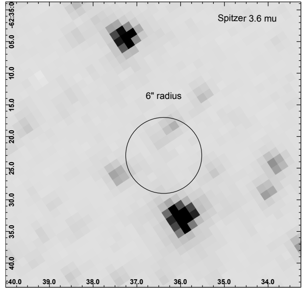
Fig. 4 Central region of the SNR observed by Spitzer in the 3.6\ \mu\text{m} band. We have overlapped the 6 arcsec extraction region used for the spectral X-ray analysis.
