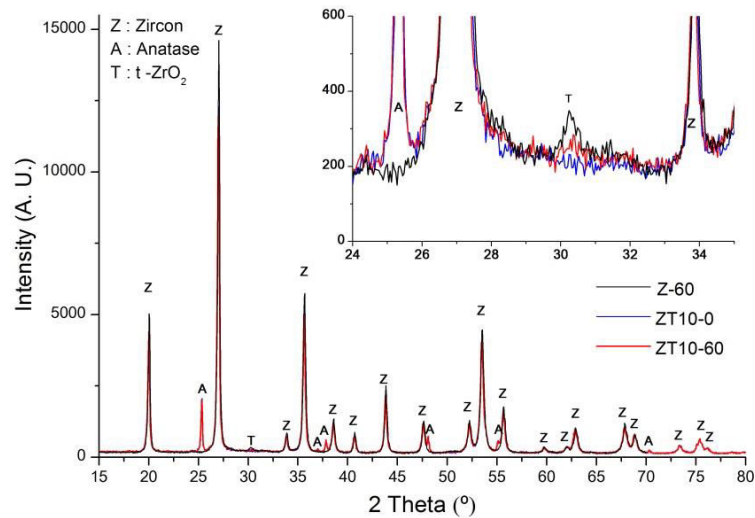
Fig. 1b. XRD patterns of the powders before (ZT10-0) and after (ZT10-60) the HEBM with 10 wt% of additive (TiO 2 ) with the milled powder of alone zircon (Z-60). (Inset: main zirconia phases peaks) [28].
