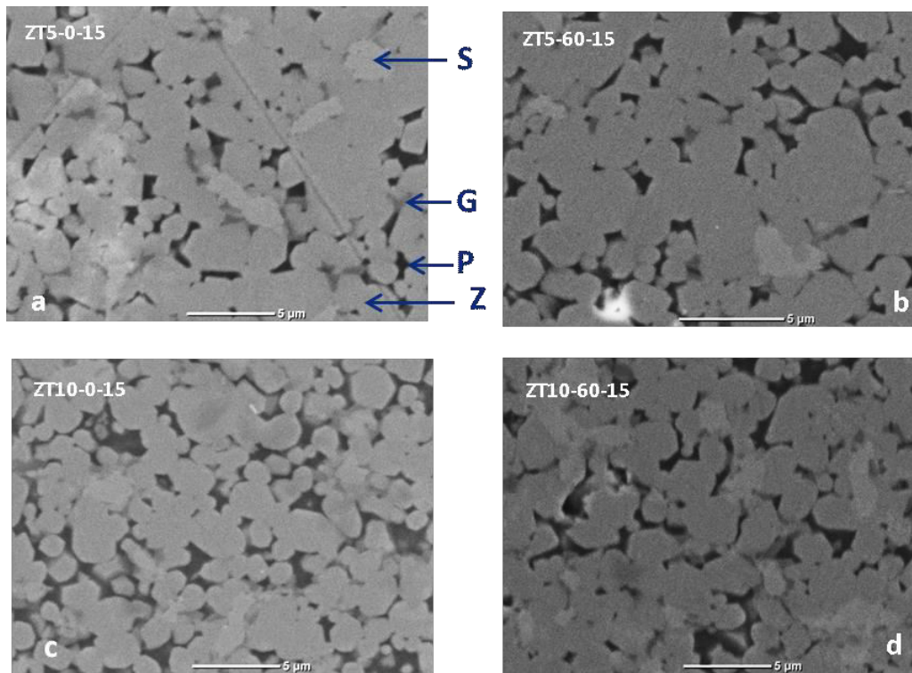
Fig. 7. SEM images of zircon – \text{TiO}_2 sintered ceramics (X2000 magnification) (see Table I for labels).
