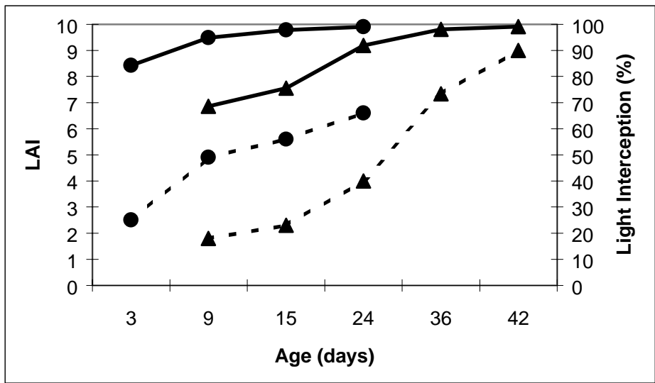
Figure 1 - Evolution of Leaf Area Index (LAI) (-----) and light Interception (—) during the longest (▲) and shortest (●) regrowth period.
