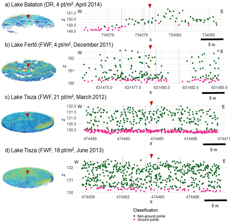
Figure 2.5. Visualization of point clouds derived from different Airborne Laser Scanning (ALS) datasets for three Hungarian lakes. (a) Lake Balaton (discrete return ALS data with 4 pt/m 2 ), (b) Lake Fertő (FWF ALS data with 4 pt/m 2 ), and (c-d) Lake Tisza (FWF ALS data with 21 pt/m 2 in March and 18 pt/m 2 in June). The left side shows the point clouds extracted within a 25 m radius around each field observation point (indicated with a red triangle) and visualized according to the z-value (blue indicates low vegetation height and red high vegetation height). On the right, 25 m long crossplots in West-East direction with 2 m width are shown (green: non-ground points, pink: ground points). DR = discrete return data, FWF = full waveform data, pt/m 2 = points per square meter, W = west, E = east.
