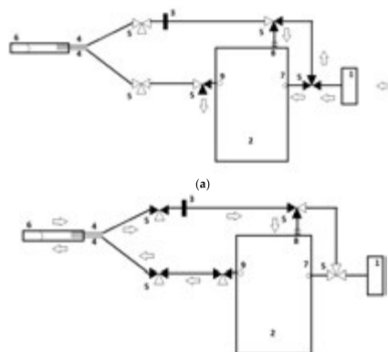
Figure 1. A schematic illustration of electronic nose setup during: (a) purging of the sensors and subsequently obtaining a baseline reference signal and (b) performing the actual sample measurement. A dark cone in a three-way valve (number 5) illustrates an air flow can pass, while a white cone prevents this. The arrows depict the air flow through the measurement setup. (a) First, the sensors are purged for 90" with filtered air derived from ambient air passing the A1-filter. The airflow, containing the residual volatile organic compounds (VOC), detached from the sensors, and is expelled through the exhaust port. Subsequently, a baseline reference signal is obtained in 30" using filtered air. (b) After the baseline reference signal is obtained, the actual measurement takes place in 60". By rotating several three-way valves, a closed loop in connection with the fecal sample is formed (6) . This loop prevents dilution of fecal VOCs with ambient air and, moreover, causes a continuous flow of fecal VOC passing the sensors. After the measurement, the three-way valves are rotated back to their original positions (Figure 1a) and the sensors are purged. (1) A1 filter, (2) Cyranose320®, (3) Polyethersulfone filter, (4) blunt needle, (5) three-way valve, (6) a vacutainer containing feces, (7) purge inlet, (8) sensor inlet, (9) exhaust portal, and (10) oxygen hose. Adapted with permission from Berkhout et al., 2016, Supplementary Material [54].
