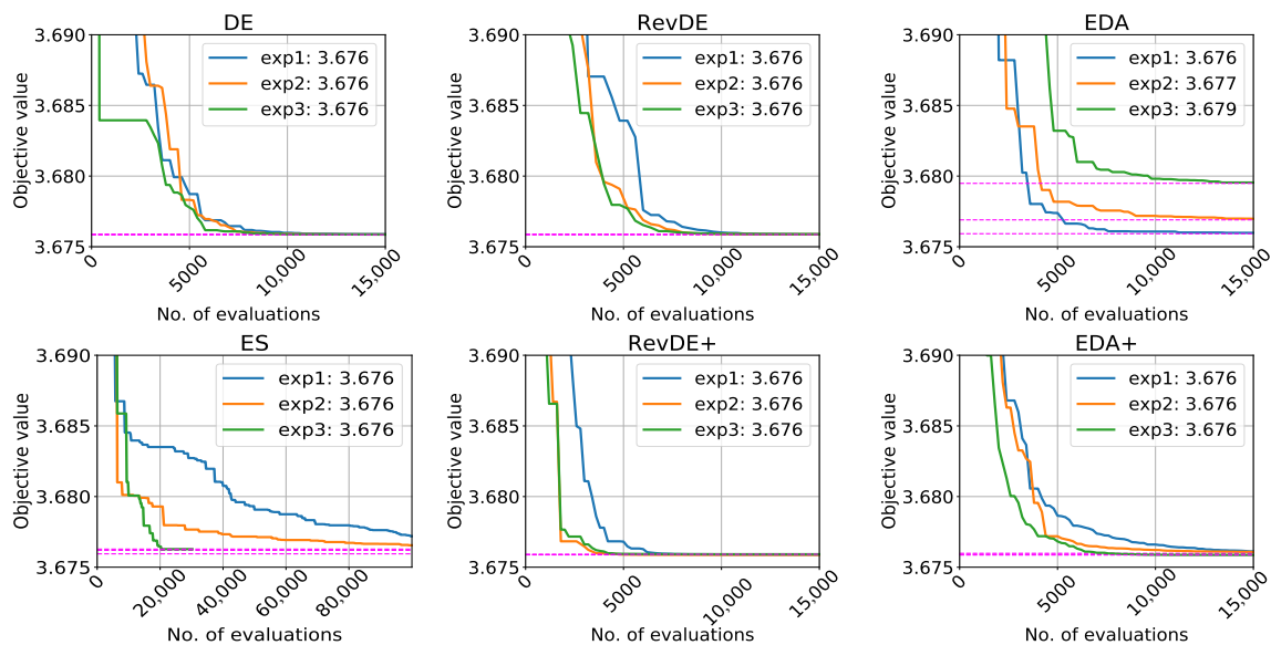
Figure 4. The convergence of the population-based optimization methods over 3 runs. In the legends, we indicate the value of the fitness function after the methods converged.
