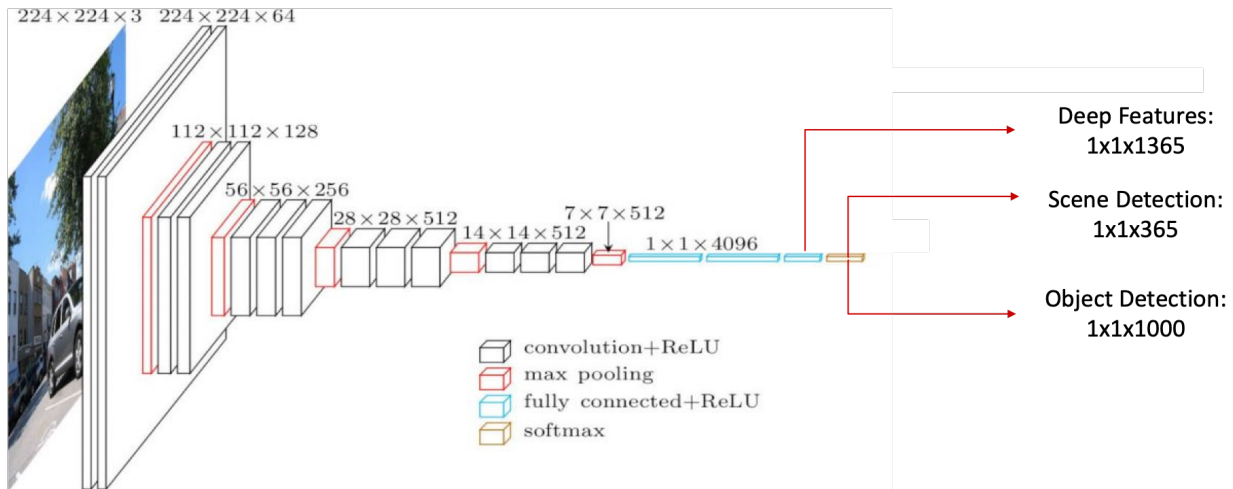
Figure 1. The VGG16 architecture [16] and an illustration of the three types of features. The deep features come from the output of the last fully connected layer of a hybrid network trained on both Imagenet [17] and places 365 [15].
