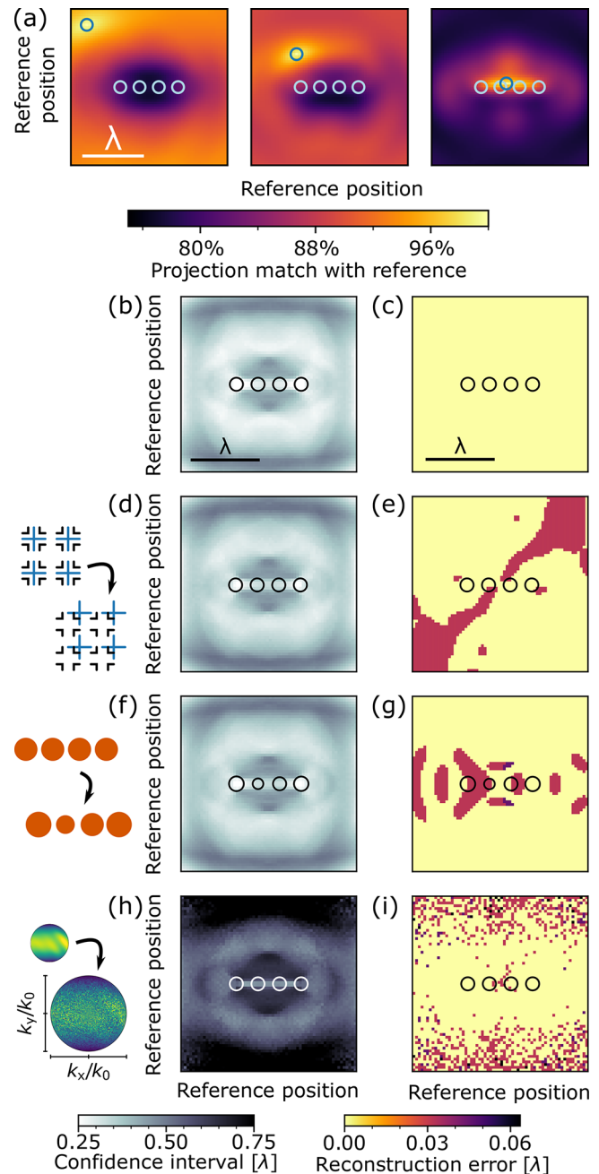
Figure 3. Position retrieval using a library. (a) Match between library and ideal data vs reference position for three different light source positions, marked with blue circles. White circles indicate array element positions. (b–i) Localization confidence interval and sample position reconstruction error vs reference position for four types of data. (b, c) Ideal data. (d, e) Sample positions displaced 30% of a library step to the north and east with respect to library positions. (f, g) Sample data taken with array elements randomly changed in diameter by up to 5%. Circles sized proportionally to element scattering strength. (h, i) Sample data degraded by shot noise as for a signal with an average of three counts per pixel, as shown to the left of (h).
