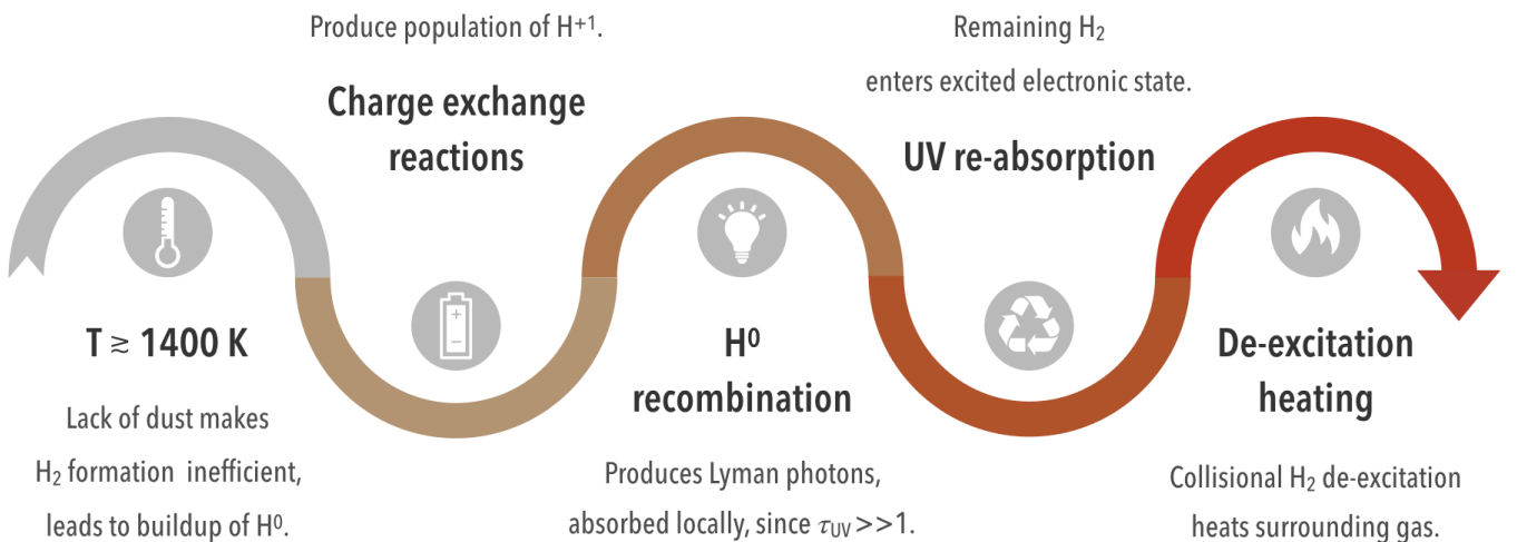
Fig. B.1. Flowchart of the inner disk physical processes leading to the high temperatures and domination of H over H 2 and C over CO at the disk midplane, in contrast to the typical photon-dominated region physics seen in molecular clouds and the upper layers of the outer disk.
