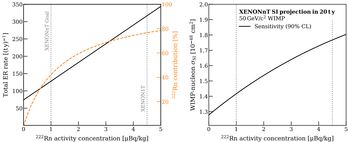
Figure 7: (Left) ER background rate in the (3, 100) cSI observable ROI as a function of the ^{222}\text{Rn} concentration in LXe. The orange dashed line represents the ^{222}\text{Rn} fractional contribution to the total ER background. The dotted grey lines indicate the XENONnT goal of 1\ \mu\text{Bq/kg} and the 4.5\ \mu\text{Bq/kg} ^{222}\text{Rn} concentration achieved in XENON1T [20]. (Right) Projection of the XENONnT sensitivity to spin-independent couplings of a 50\ \text{GeV}/c^2 WIMP under varying assumptions on the ^{222}\text{Rn} concentration.
