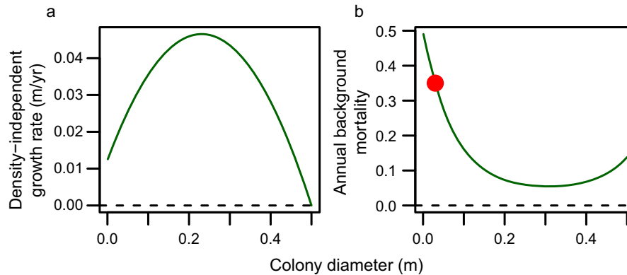
FIG. 1. Growth and mortality functions used in the model. (a) Density-independent growth rate in m/yr vs. colony diameter. This plot shows g_0 , the growth rate in uncrowded conditions. (b) Annual mortality vs. colony diameter, based on data for corymbose colonies reported in Madin et al. (2014), and adjusted to match 35% small-colony mortality for x = 0.03 m colonies reported in Holbrook et al. (2018) (shown by the point in red). This plot shows annual mortality as a proportion, although mortality enters the model as the equivalent rate.
