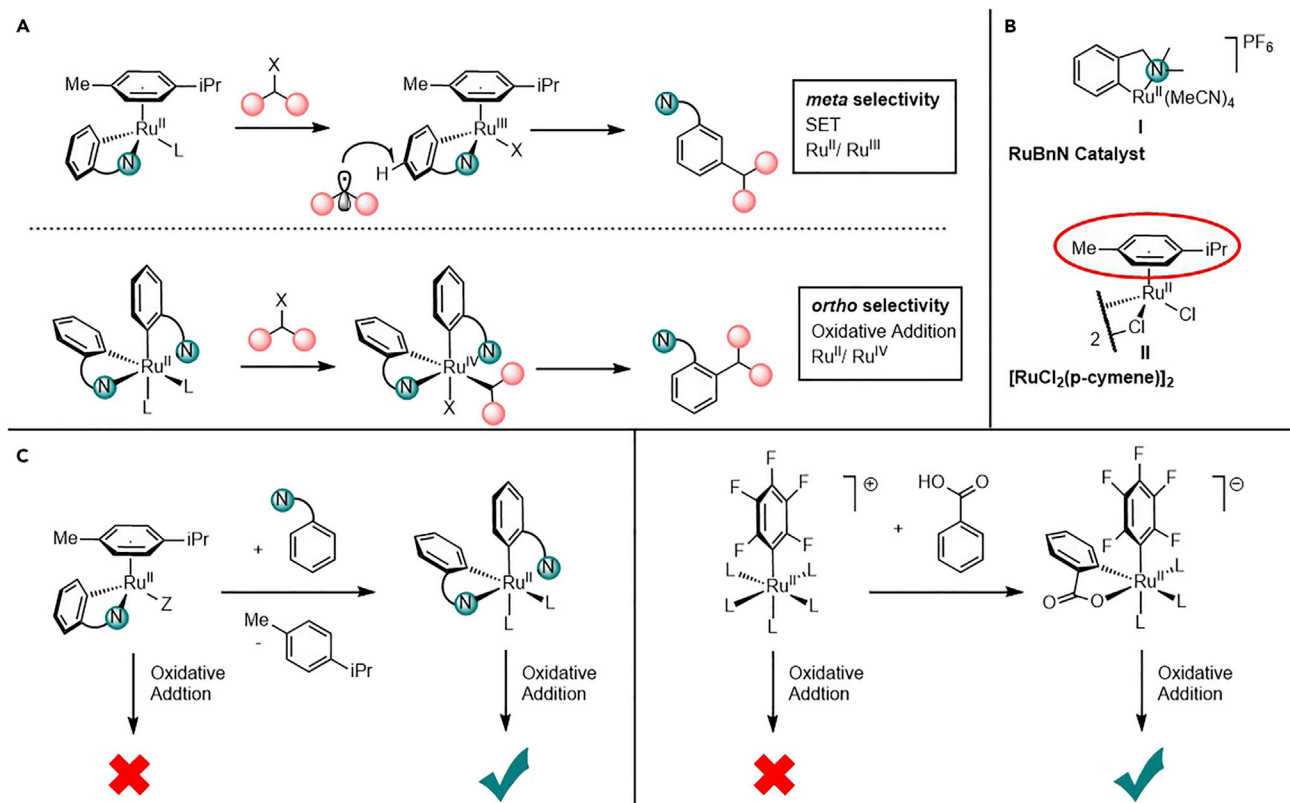
Figure 1. Ru-Catalyzed C–H Functionalization
