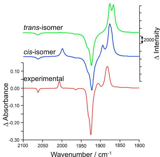
Fig. 2. The red spectrum is the experimental difference spectrum obtained following steady-state ( \lambda_{\text{exc}} = 395 nm) photolysis of [(\text{CO})_5\text{WC}(\text{NC}_4\text{H}_8)\text{Me}] in n -pentane solution in the presence of a trapping ligand ( \text{PPh}_3 , in 1.1 molar equivalent excess). The blue spectrum is the calculated spectrum of cis - [(\text{CO})_4(\text{PPh}_3)\text{WC}(\text{NC}_4\text{H}_8)\text{Me}] minus the spectrum of [(\text{CO})_5\text{WC}(\text{NC}_4\text{H}_8)\text{Me}] and the green spectrum represents the calculated spectrum of trans - [(\text{CO})_5\text{WC}(\text{NC}_4\text{H}_8)\text{Me}] minus the spectrum of [(\text{CO})_5\text{WC}(\text{NC}_4\text{H}_8)\text{Me}] . All calculated spectra were modelled in n -heptane.
