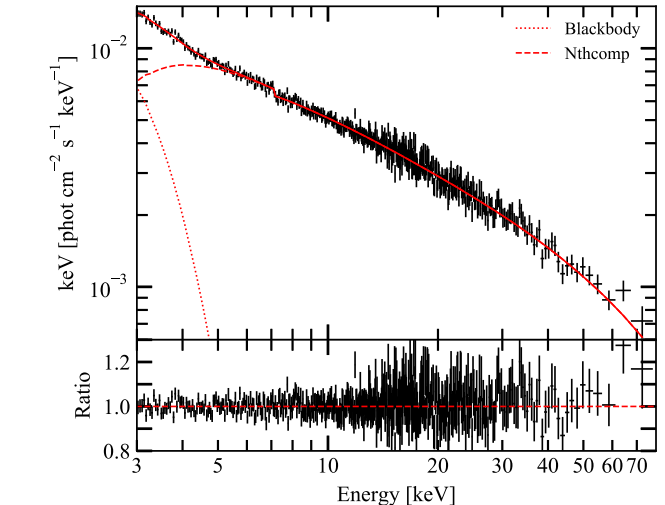
Figure 5. Top: the 2018 NuSTAR spectrum of 4U 1608–52, unfolded around the best-fitting TBABS×(BBODYRAD+NTHCOMP) continuum model using the XSPEC command EUFSPEC. The data have been visually rebinned for clarity to an S/N>10. The red dotted, dashed, and solid lines show the thermal, Comptonized, and total model, respectively. Bottom: data-to-model ratio for the continuum model shown in the top panel.
