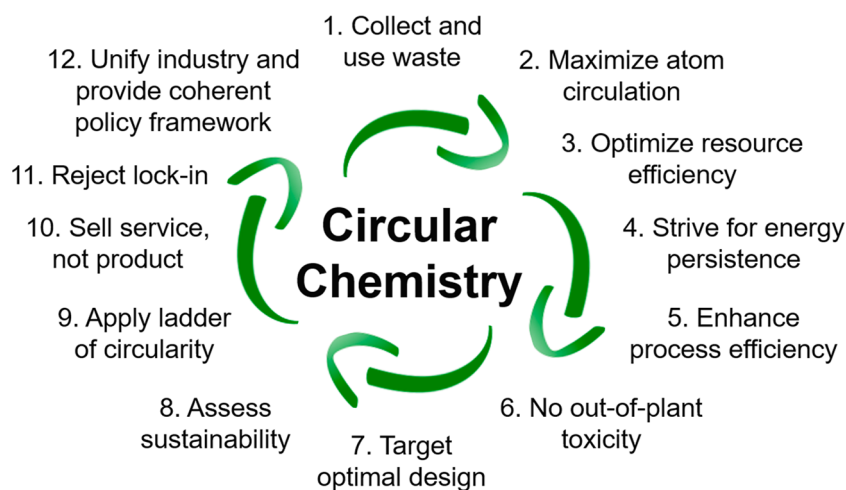
Figure 2. Twelve principles of circular chemistry. Reproduced with permission from ref 36. Copyright 2019 Springer Nature.
