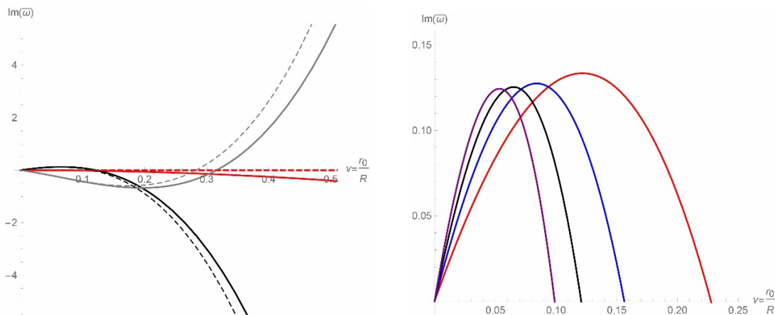
Figure 6. The left plot exhibits the behaviour of the imaginary part of the frequencies \omega_2 (red solid line), \omega_3 (black solid line) and \omega_4 (grey solid line) for black rings up to second order in derivatives as a function of the ring thickness \nu = r_0/R for D = 7 and m = 10 . The dashed lines are the corresponding frequencies for boosted black strings in (3.12) with critical boost. The right plot exhibits the growth rate of the instability associated to \omega_3 as a function of \nu for m = 6 (red line), m = 8 (blue line), m = 10 (black line) and m = 12 (purple line).
