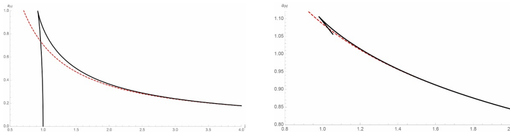
Figure 1. On the left we show the reduced area a_H as a function of the reduced angular momentum j for D = 5 where the black line is the exact curve of the black ring solution [27] and the dashed red curve is the blackfold approximation up to first order in derivatives [28]. On the right we show the behaviour of the same quantities for black rings in D = 7 where the black line is the numerical solution of [29] and the dashed red line the blackfold approximation up to second order in derivatives [30].
