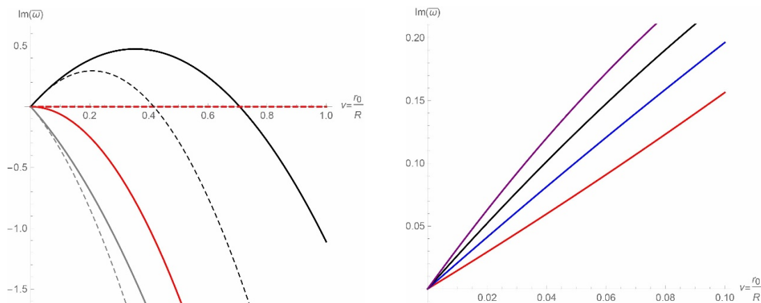
Figure 5. On the left, we show the imaginary part of frequencies \omega_2 (red solid line), \omega_3 (black solid line) and \omega_4 (grey solid line) for black rings up to first order in derivatives as a function of the ring thickness \nu = r_0/R for D = 5 and m = 10 using the full expressions provided in the supplementary material. The dashed lines are the corresponding frequencies for boosted black strings in (3.7) with critical boost. On the right plot we show the behaviour of the imaginary part of \omega_3 as a function of m for m = 6 (red), m = 8 (blue), m = 10 (black) and m = 12 (purple) for D = 5 .
