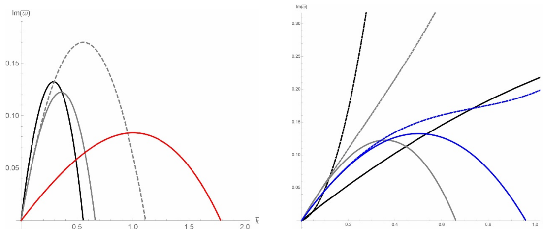
Figure 3. The figure on the left exhibits the imaginary part of \omega_3 at second order using (C.1) as a function of \bar{k} for D = 7 for different values of the boost parameter: \beta = 0 (black solid line), \beta = 1/2 (grey solid line) and \beta = 9/10 (red solid line). The grey dashed line represents the first order result for \beta = 1/2 obtained in (3.7). The figure on the right provides a comparison between blackfold and large D results for D = 5 and D = 7 for static strings and at the critical boost. The blue solid line is the blackfold result at second order for \beta = 0 and D = 7 while the dashed line is the corresponding large D result at fourth order derived in [40]. The black solid line represents the imaginary part of \omega_3 at first order as in (3.7) while the black dashed line is the corresponding result at large D [24]. The grey solid line is the imaginary part of \omega_3 as in (C.1) while the grey dashed line is the corresponding large D result (C.2).
