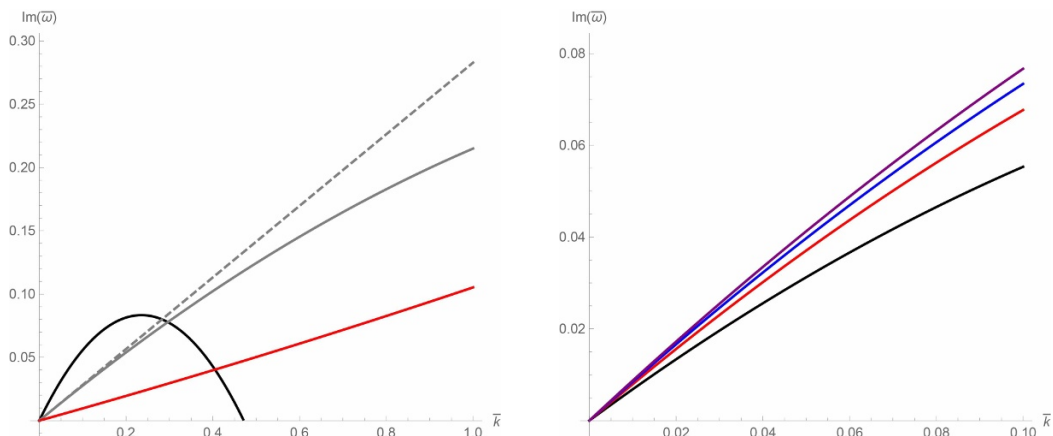
Figure 2. On the left we show the dimensionless imaginary part of \omega_3 , defined as \bar{\omega} = \text{Im}\omega_3 r_0 , as a function of \bar{k} = kr_0/\sqrt{n} for D = 5 ( n = 1 ). The black solid line represents \beta = 0 , the grey solid line \beta = 1/\sqrt{2} and the red solid line \beta = 9/10 while the grey dashed line is the imaginary part of the ideal order result (3.5). We have shown these curves up to \bar{k} = 1 , but we only expect them to be strictly valid for small \bar{k} . On the right plot we show the behaviour of the imaginary part of \omega_3 for \beta = 1/10 and n = 1 (black), n = 2 (red), n = 3 (blue) and n = 4 (purple).
