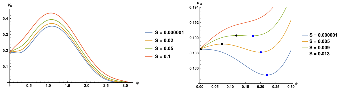
FIG. 1. Plots of the effective potential at fixed entropy V_s , as a function of the angle \psi on S^3 . Both figures represent plots at p/M = 0.03 . The right plot zooms into the region near the North pole of the S^3 . As we increase the entropy we encounter a critical value S^* , where the metastable vacuum of KPV (blue dots on the right) merges with a new unstable vacuum (black dots on the left).
