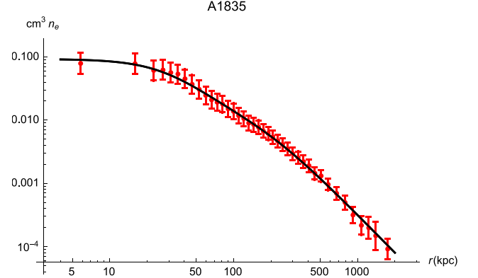
Figure 3. Data for n_e in A1835 and their best fit (10) with (11).
