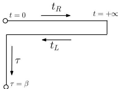
Figure 1. The Schwinger-Keldysh contour at finite temperature. Time flows forward from t = 0 to t = +\infty and back to where the initial state is defined. The latter is represented by an imaginary time segment identified along the circles with period \beta = 1/T .
