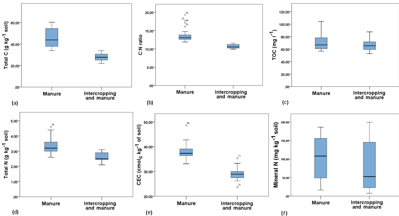
Figure 2. Boxplots showing the differences between (a) total C (g kg -1 soil), (b) C/N ratio, (c) total organic C in the extracts (mg L -1 ), (d) total N (g kg -1 soil), (e) cation exchange capacity (CEC in cmol c kg -1 ), and (f) mineral N (mg kg -1 soil) for the agricultural management practices of manure and intercropping and manure.
