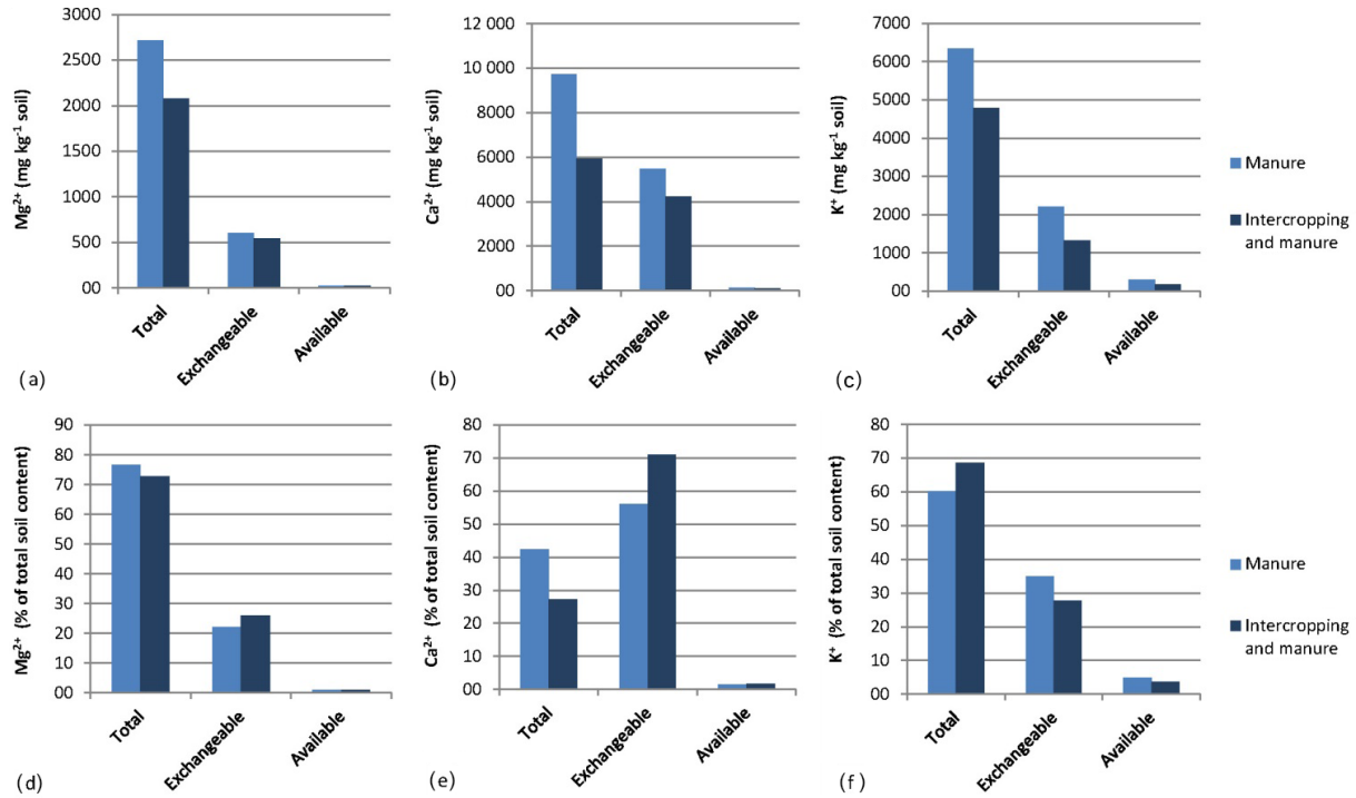
Figure 1. (a, b, c) Bars length show the total, exchangeable, and plant available / water-soluble amount of Mg, Ca, and K (in mg kg -1 soil) under management practices of manure and intercropping and manure. (d, e, f) Total, exchangeable, and plant available / water-soluble Mg, Ca, and K in the soil as percentage of the sum.
