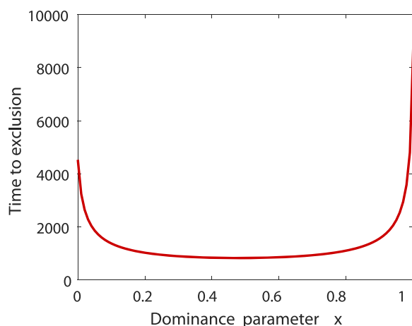
Fig. 5. The effect of incomplete dominance on the time to allele fixation. At x = 0 the resistant allele is dominant; at x = 1 the susceptible allele is dominant.
