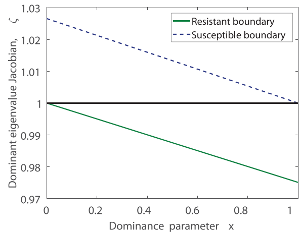
Fig. 4. The effect of incomplete dominance on boundary stability as measured by the dominant eigenvalue of the Jacobian. At x = 0 the resistant allele is completely dominant, and at x = 1 the susceptible allele is completely dominant.
