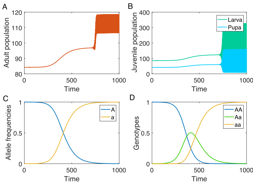
Fig. 1. Eco-evolutionary dynamics of the invasion of an allele with a higher fecundity \beta ( \beta_{AA} = 5.68 , \beta_{Aa} = 8.68 , \beta_{aa} = 11.68 ). All other parameters are taken from Table 1 in Dennis et al. (1995) and are set equal for all three genotypes: \chi_i = 0.009264 , \xi_i = 0.01097 , \kappa_i = 0.01779 , \mu_i = 0.5129 , \nu_i = 0.1108 for all i . a. Abundance of the adult stage. b. Abundance of larvae and pupae. c. Frequencies of the A and a alleles. d. Frequencies of the three genotypes.
