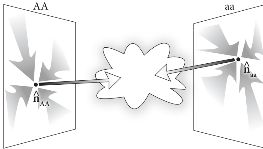
Fig. 2. Graphical depiction of the \omega g -dimensional space defined by combinations of \omega stages and g genotypes. If both the homozygous boundaries are unstable, then a homozygote state can never be reached again once both alleles are present in the population (since both alleles grow when rare). Image by Jan van Arkel.
