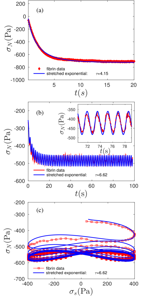
FIG. 5. Fibrin gels polymerized at 22°C. (a) The red line shows the normal stress relaxation versus time for a constant shear stress. The blue line is a stretched exponential fit to the data, which yields the relaxation time \tau = 4.15 s. (b) The red line shows the normal stress versus time for an oscillatory shear stress with frequency \nu = 0.3 Hz. The blue line is the fit using Eq. (27), which yields the relaxation time \tau = 6.62 s. The inset zooms in on the steady-state response. (c) The same data shown in (b) plotted as normal stress versus shear stress.
