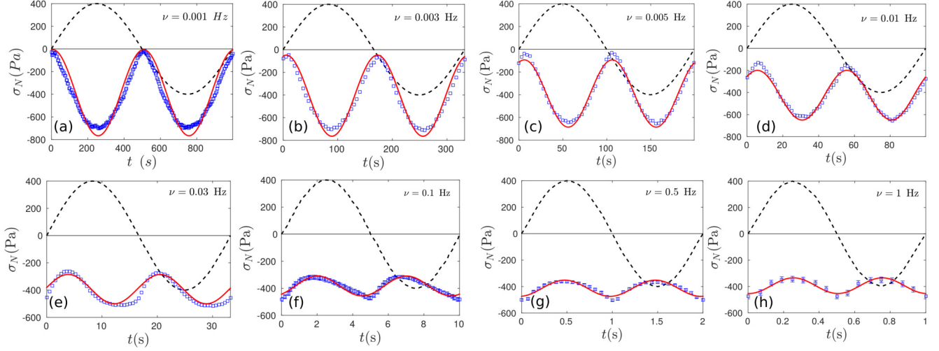
FIG. 6. Normal stress response (blue square symbols) of a fibrin gel polymerized at 27°C to an oscillating shear stress (dashed line) for different frequencies \nu versus time. The fit (red line) according to Eqs. (21)–(23) is also shown where the fitting parameters are 2A_z and \tilde{A} . In these equations the shear modulus G is independently obtained from the rheology data. The data shown at \nu > 0.1 Hz represent averages with standard deviations obtained by averaging over 34 cycles to compensate for the low sampling frequency of the rheometer. [Data in (a), (d), and (h) from Ref. [18].]
