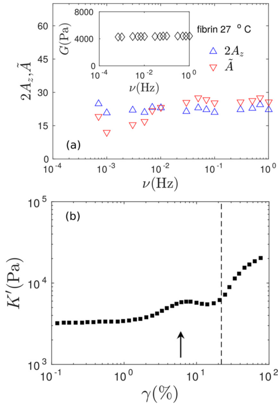
FIG. 8. (a) Fitting parameters 2A_z and \bar{A} versus frequency for a fibrin gel polymerized at 27°C. The inset shows the shear modulus versus frequency, measured independently by rheology. (b) Differential storage modulus K' as a function of applied shear strain for a fibrin gel polymerized at 27°C. The arrow indicates the onset of nonlinearity at \gamma_0 = 6.0\% , calculated using Eq. (50). The dashed line corresponds to an applied shear stress of 800 Pa, which is the applied stress in Figs. 6 and 7.
