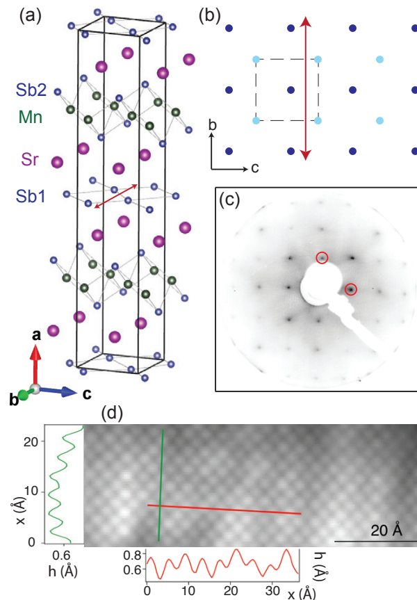
Figure 1: Bulk and surface crystallographic structure. (a): Crystal structure of \text{SrMnSb}_2 , featuring two inequivalent Sb positions, labelled as Sb1 and Sb2. The Sb1 plane is sandwiched between two staggered Sr planes. The Sb2 atoms sandwich a plane of the Mn atoms. (b): A plan view of the Sb1 plane, the key structural element of the crystal. The buckling of the Sb1 plane out of the b - c plane is indicated using different shades for the Sb1 atoms. A non-symmorphic symmetry element in the form of a screw axis is indicated as a red arrow aligned along b . (c): LEED diffraction pattern of an in-situ cleave of \text{SrMnSb}_2 , recorded with an incident electron energy of 220 eV at 30 K. The pattern is of a (1 \times 1) type, whereby the red circles highlight the (1,0) and (0,1) ( h,k ) diffraction spots. (d) STM topograph of cleaved \text{SrMnSb}_2 measured at 77 K in UHV using a Pt/Ir tip at V = -600 mV and I = 95.8 pA. The same (1 \times 1) surface symmetry is seen as in the LEED data, and the interatomic separation corresponds to the net of the Sb1 atoms.
