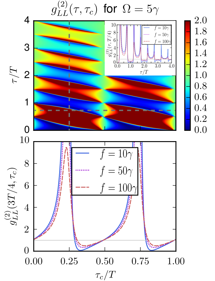
FIG. 4. (top) Second-order coherence function g_{LL}^{(2)}(\tau, \tau_c) for the sign-change protocol g(t) = g_0 \cos(\Omega t) of the moderately driven ( f = 10\gamma ) qubit on resonance ( \delta = 0 ) at fast modulation frequency \Omega = 5\gamma . The oscillations decay with the delay time \tau at the rate \gamma as can be seen, e.g., along the vertical cut at \tau_c = T/4 shown in the inset. Thus, this rapidly changing behavior takes place only for sufficiently fast modulations. (bottom) The strong oscillations in time \tau_c between bunching and antibunching behavior reported in Ref. [37] become less pronounced with increasing input power f as the qubit becomes saturated. The delay time \tau is fixed at the value 3T/4 , which corresponds to the horizontal cut in the top figure.
