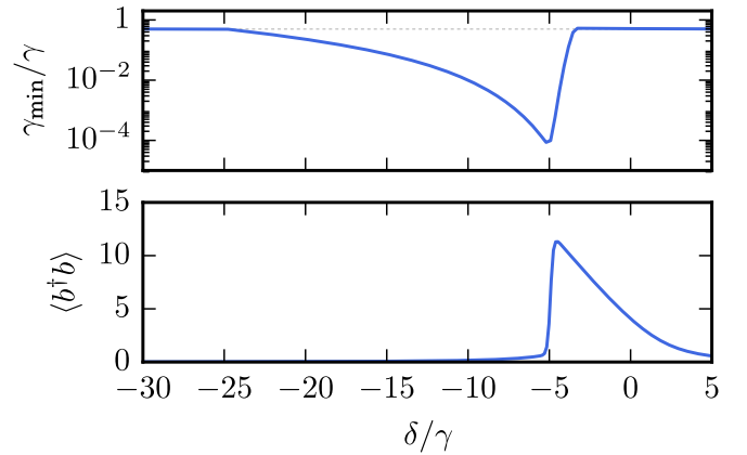
FIG. 7. (top) Smallest dissipation rate \gamma_{\min} of the undriven Kerr-nonlinear model as a function of detuning \delta for U = -\gamma/2 and f = 16\gamma . Similar to the two- and three-level systems, the smallest dissipation rate is significantly suppressed within the critical region, although it remains finite. (bottom) One of the important signatures of the dissipative phase transition is a prominent increase in the stationary occupation number \langle b^\dagger b \rangle which peaks at the same parameter value for which the minimal dissipation rate is reached. In the following, the periodic modulation of \delta is considered across the whole critical region with modulation frequency \Omega \ll \gamma .
