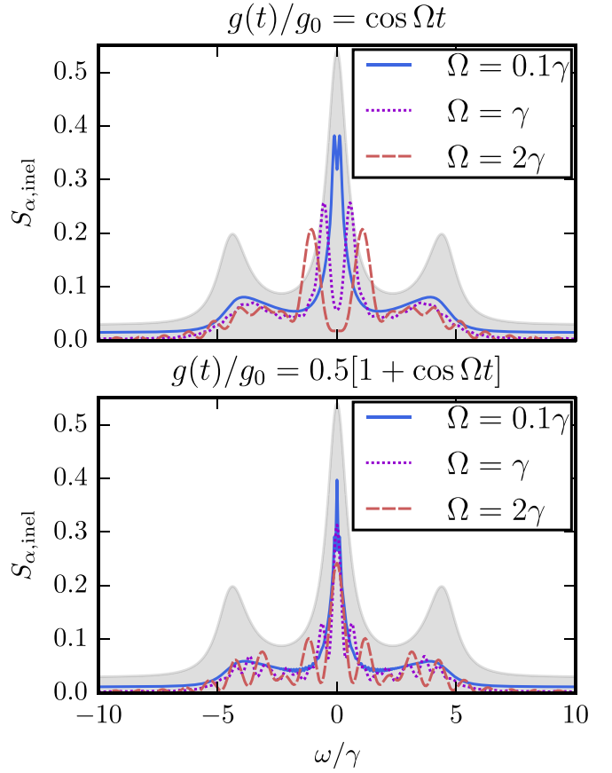
FIG. 3. Inelastic power spectra of the qubit strongly driven ( f = 200\gamma ) on resonance ( \delta = 0 ) for the (top) sign-change protocol g(t) = g_0 \cos \Omega t and the (bottom) on-off protocol g(t) = \frac{g_0}{2}(1 + \cos \Omega t) for various modulation frequencies \Omega . The Mollow triplet for the corresponding stationary case at coupling g = g_0 is shown for comparison in gray. Additional broadened peaks consistent with the Floquet spectrum arise due to the periodic modulation and may destructively interfere as seen, for example, in the missing main peak in the case of the sign-change protocol (top). Similar features in the power spectrum have been reported in Ref. [40] for a qubit subject to a pulsed excitation.
