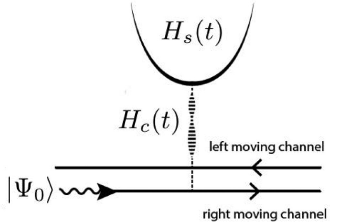
FIG. 1. Open quantum system model: A local system is coupled to a transmission line supporting left- and right-propagating modes. Either the system's parameters or its coupling to the transmission line is periodically modulated. The input pulse into the transmission line is given by a coherent state |\Psi_0\rangle in the right-propagating mode \omega_0 . The pulse's intensity is characterized by the photonic flux f .
