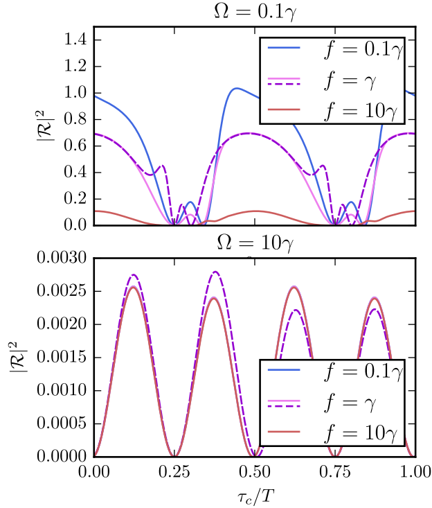
FIG. 2. Reflection from the qubit on resonance, \delta = 0 , for the time-modulated coupling g(t) = g_0 \cos \Omega t with slow \Omega = 0.1\gamma (top) and fast \Omega = 10\gamma (bottom) modulation frequencies, expressed in the units of \gamma = \pi g_0^2 . (top) The adiabatic approximation (dashed line) obtained from Eq. (19) deviates from the numerical solution in the vicinities of time instants when the coupling is quenched. For all values of f , the reflection is suppressed at these points. At large f , the reflection is completely suppressed because of the qubit's saturation. (bottom) The high-frequency modulation suppresses the reflection for any input power f . The numerical result (solid lines) is well approximated by the high-frequency result (dashed line) obtained from Eqs. (25)–(27).
