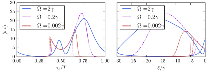
FIG. 8. (left) Periodic steady-state occupation \langle b^\dagger b \rangle(t) of the Kerr-nonlinearity model under periodic modulation of detuning \delta(t) = -15\gamma[1 + \cos \Omega t] for various modulation frequencies \Omega . (right) The same dependence in the parametric representation. For moderate modulation frequencies, the occupation is strongly enhanced compared with the true stationary state shown in the lower panel of Fig. 7. The adiabatic approximation based on Eq. (19) is given by the light brown curve (note that in the parametric representation it lies very close to the stationary-state result). The numerical results for rather small frequency \Omega = 0.002\gamma (brown) still drastically deviate from the corresponding adiabatic approximation (light brown). As discussed by Casteels et al. [31], the dynamical hysteresis seen in the parametric plot is directly related to the breakdown of adiabaticity in the critical region, and the hysteresis area depends on the width of the parameter range where \Omega > \gamma_{\min} .
