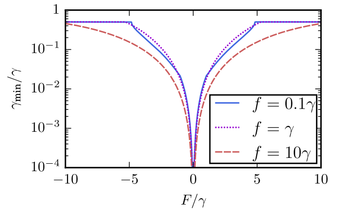
FIG. 5. Smallest dissipation rate \gamma_{\min} of the \Lambda system as a function of the classical drive field amplitude F . Instead of directly modulating the coupling strength g , the three-level \Lambda system allows tuning of \gamma_{\min} by means of F . The input power f of the probe field has little effect on this behavior.
