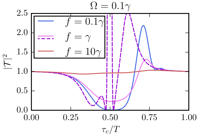
FIG. 6. Transmission through the \Lambda system which is driven on resonance ( \delta_1 = \delta_2 = 0 ) by both probe and drive pulses. The drive field has a periodically modulated amplitude F(t) = 10\gamma[1 + \cos \Omega t] at \Omega = 0.1\gamma . The adiabatic approximation (dashed line) is only valid far away from the critical region defined by \Omega > \gamma_{\min} (cf. Fig. 5). In the time window where it breaks down, the system responds nonadiabatically. At large powers f of the probe field, these effects are, however, washed out because of the system's saturation.
