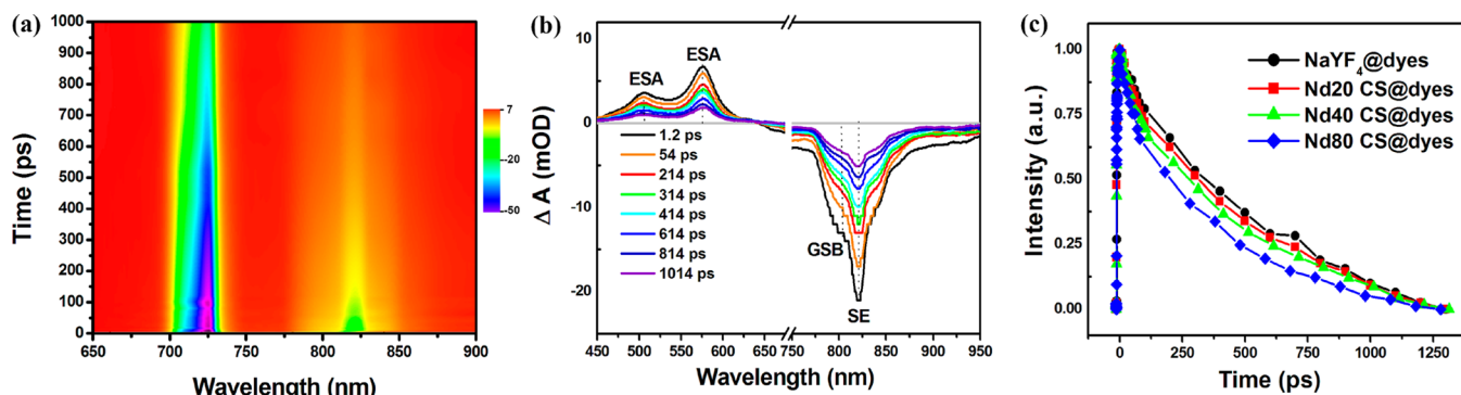
Figure 3. (a) Top view of TA data of dye-sensitized Nd20 CS UCNP in \text{CHCl}_3 . (b) Relative absorption variation as a function of the wavelength for time delays ranging from 1.2 to 1014 ps with 720 nm pumping for Nd20 CS UCNP. (c) Time-resolved TA spectra of dye-linked \text{NaYF}_4 nanoparticles, dye-sensitized Nd20 CS, dye-sensitized Nd40 CS, and dye-sensitized Nd80 CS probed at 825 nm; all of the samples kept \sim 2600 dye molecules per nanoparticle.
