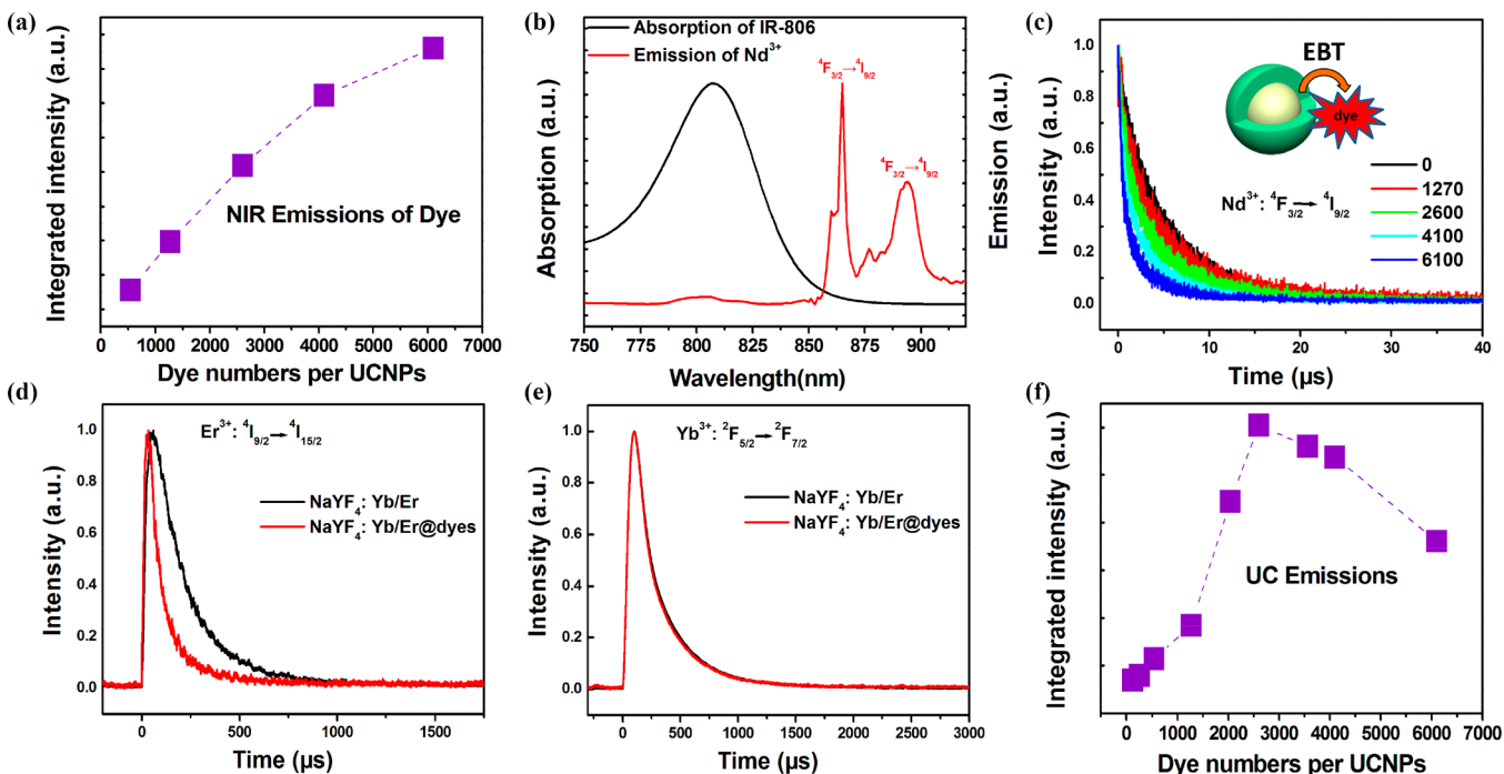
Figure 2. (a) NIR emission intensity integrated in the range of 810 to 870 nm of IR-806 sensitized UCNPs as a function of the conjugated dye numbers per UCNP. (b) Emission spectrum of Nd 3+ and absorption spectrum of IR-806. (c) Luminescence decay curves of Nd 3+ emission in the Nd 20 CS at 863 nm with variable conjugated dyes (0–6100 per UCNP). (d) Lifetimes of Er 3+ ( 4 I 9/2 → 4 I 15/2 , emission at ~800 nm) of NaYF 4 :Yb/Er nanoparticles without dyes (black lines) and with dyes (red line, ~3000 dyes per UCNP) under 980 nm excitation. (e) Lifetimes of Yb 3+ ( 2 F 5/2 → 2 F 7/2 , emission at ~1040 nm) of NaYF 4 :Yb/Er nanoparticles without dyes (black lines) and with dyes (red line, ~3000 dyes per UCNP) under 980 nm excitation. (f) UCL intensity integrated in the range of 500–700 nm of IR-806 sensitized UCNPs as a function of the linked dye numbers per UCNP.
