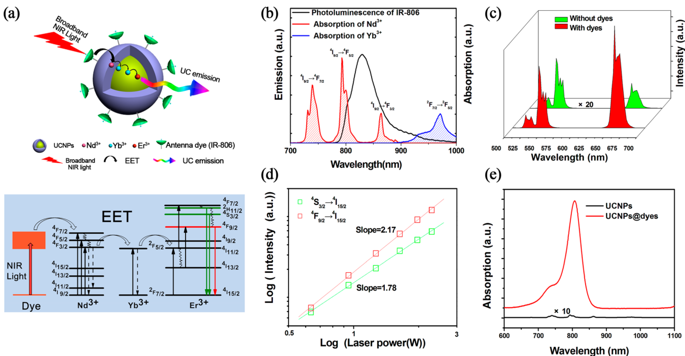
Figure 1. (a) Schematic diagram illustrating the UCL of IR-806 sensitized core–shell UCNPs based on an excitation energy transportation mechanism and simplified energy-level diagrams illustrating the energy-transfer process. Key: EET: excitation energy transportation; NIR: near-infrared; and UC: upconversion. (b) Emission spectrum of IR-806 under excitation of 808 nm in CHCl 3 (black line), absorption spectra of Nd 3+ (red line), and Yb 3+ (blue line). (c) UCL of Nd 20 CS and the dye-sensitized Nd 20 CS under an excitation of 808 nm (8.3 W/cm 2 ). (d) Log–log plots of the UCL intensity versus laser power for the green and red emissions of the dye-sensitized Nd 20 CS under excitation of 808 nm. (e) Absorption spectra of Nd 20 CS (black line) and dye-sensitized Nd 20 CS.
