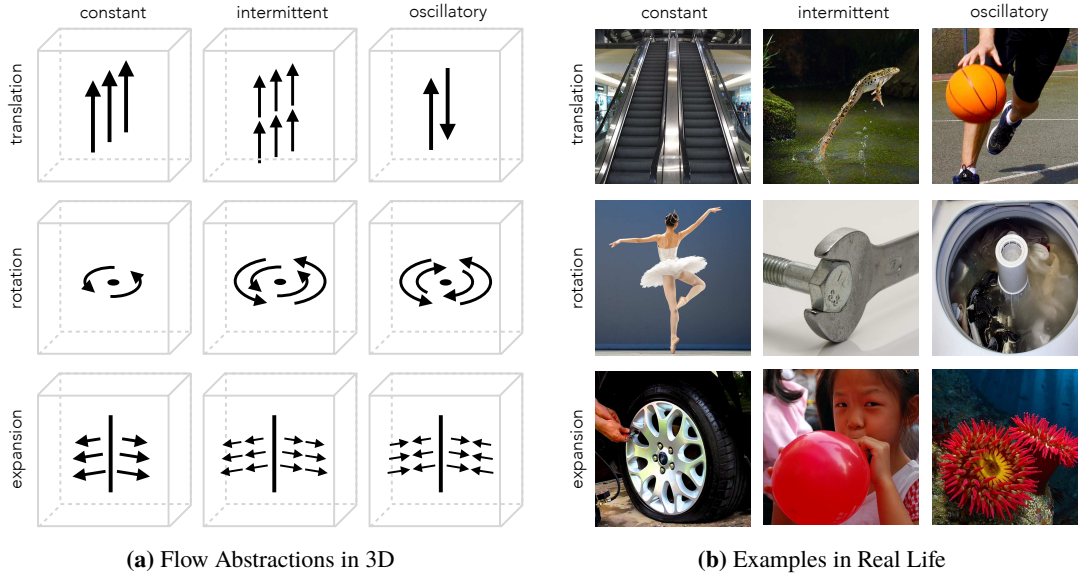
Figure 2. 3 \times 3 Cartesian table of the motion type times the motion continuity . Following from the differential operators acting on the flow, these are the basic cases of (periodic) motion in 3D. The examples are: escalator, leaping frog, bouncing ball, pirouette, tightening a bolt, laundry machine, inflating a tire, inflating a balloon and a breathing anemone. Figure originally appeared in [3].
