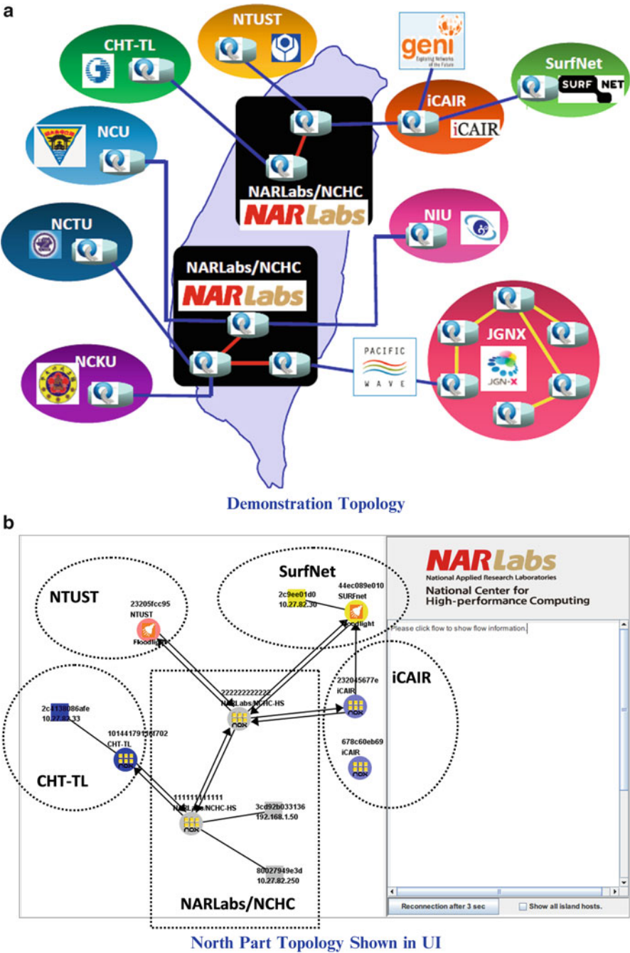
Fig. 15 Multi-domain automatic network topology discovery in SC13 demonstration
