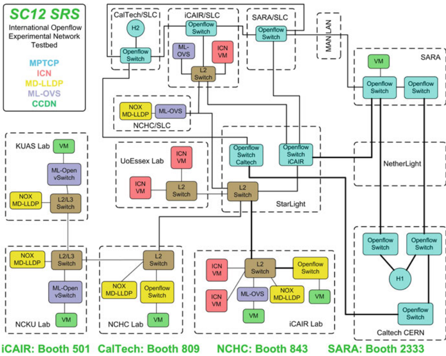
Fig. 6 International advanced network research facility segmented by project at SC12
