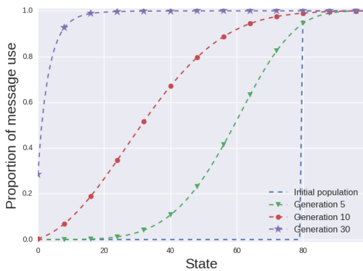
Figure 3: Noisy iterated learning ( \gamma = 1 , \sigma = 0.4 , k = 30 ).
