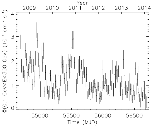
Fig. 2. Light curve of the integral fluxes between 0.1 and 300 GeV in bins of ten days measured with Fermi -LAT. The dashed line indicates the average flux.
